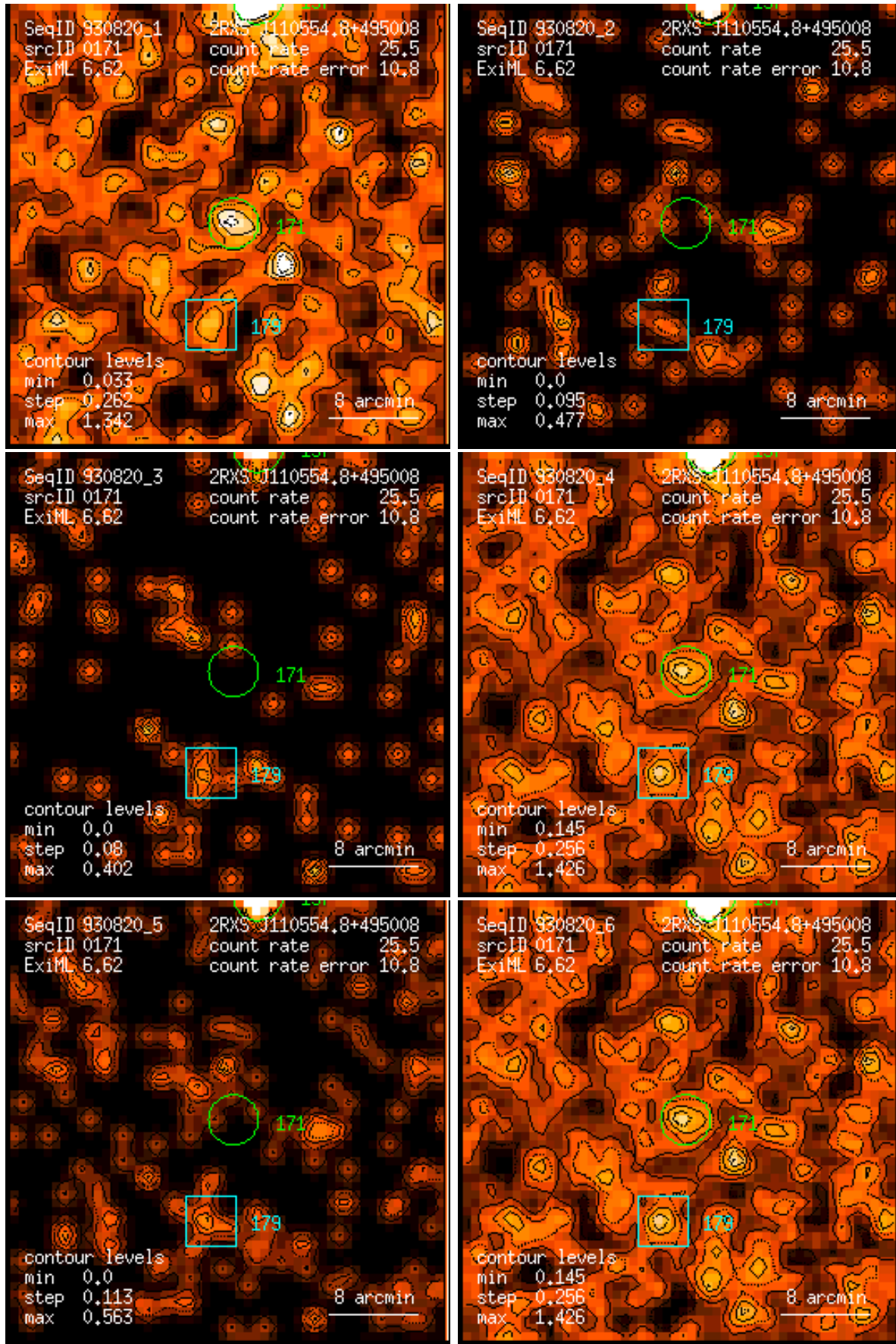
Figure 171: RASS 930820: detection 0171: band rate images, Gaussian filter: (1) PSPC channels 11 – 41, (2) 52 – 90, (3) 91 – 201, (4) 11 – 235, (5) 52 – 201, (6) 11 – 201. Broad band rates in counts/ks. Band rate contour levels in counts/ks/arcmin 2 .
