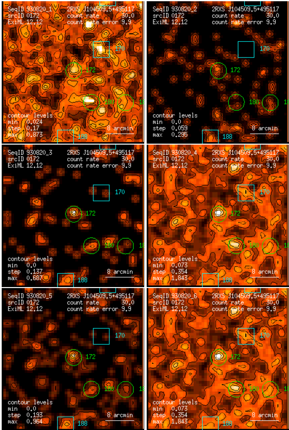
Figure 172: RASS 930820: detection 0172: band rate images, Gaussian filter: (1) PSPC channels 11 – 41, (2) 52 – 90, (3) 91 – 201, (4) 11 – 235, (5) 52 – 201, (6) 11 – 201. Broad band rates in counts/ks. Band rate contour levels in counts/ks/arcmin 2 .
