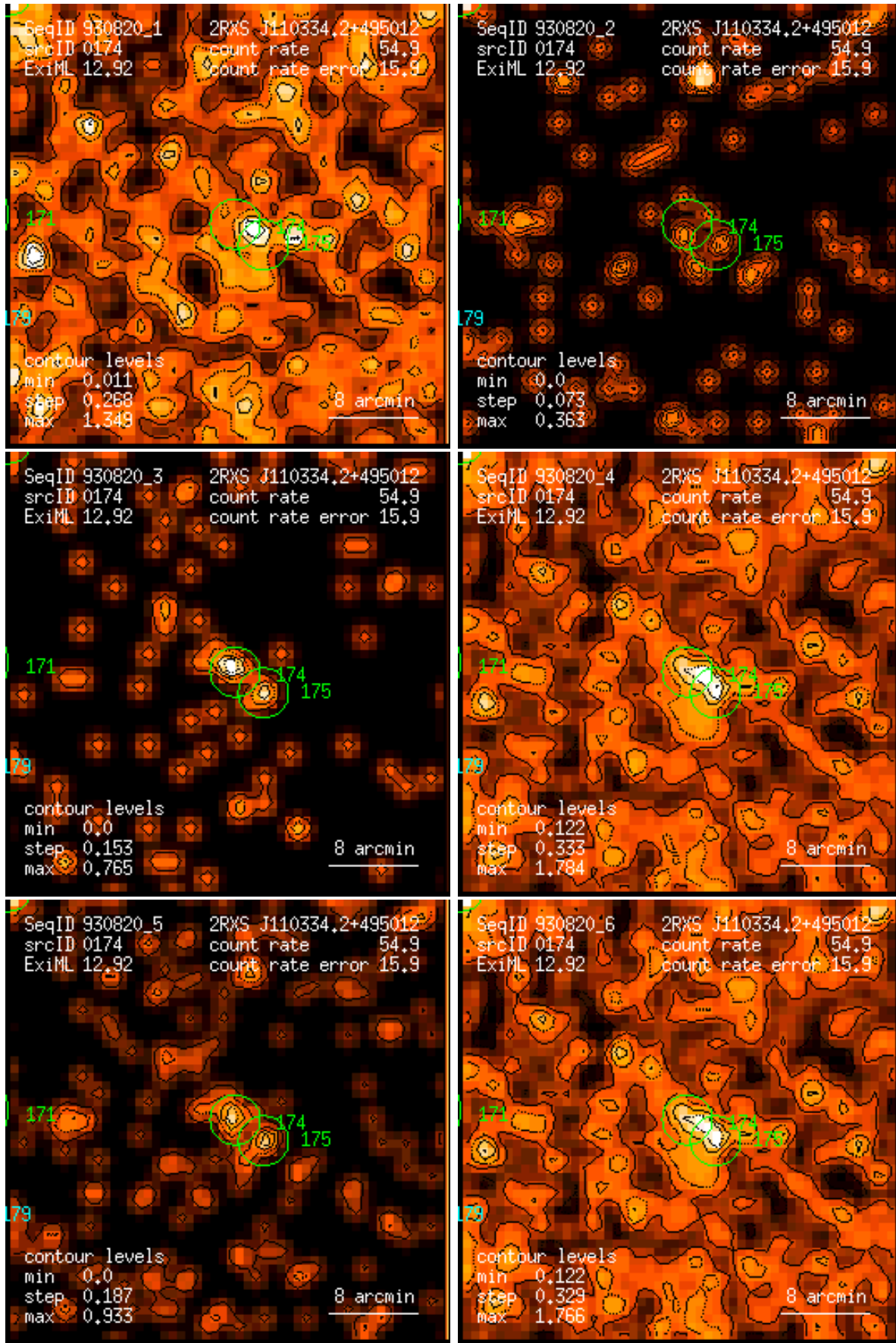
Figure 174: RASS 930820: detection 0174: band rate images, Gaussian filter: (1) PSPC channels 11 – 41, (2) 52 – 90, (3) 91 – 201, (4) 11 – 235, (5) 52 – 201, (6) 11 – 201. Broad band rates in counts/ks. Band rate contour levels in counts/ks/arcmin 2 .
