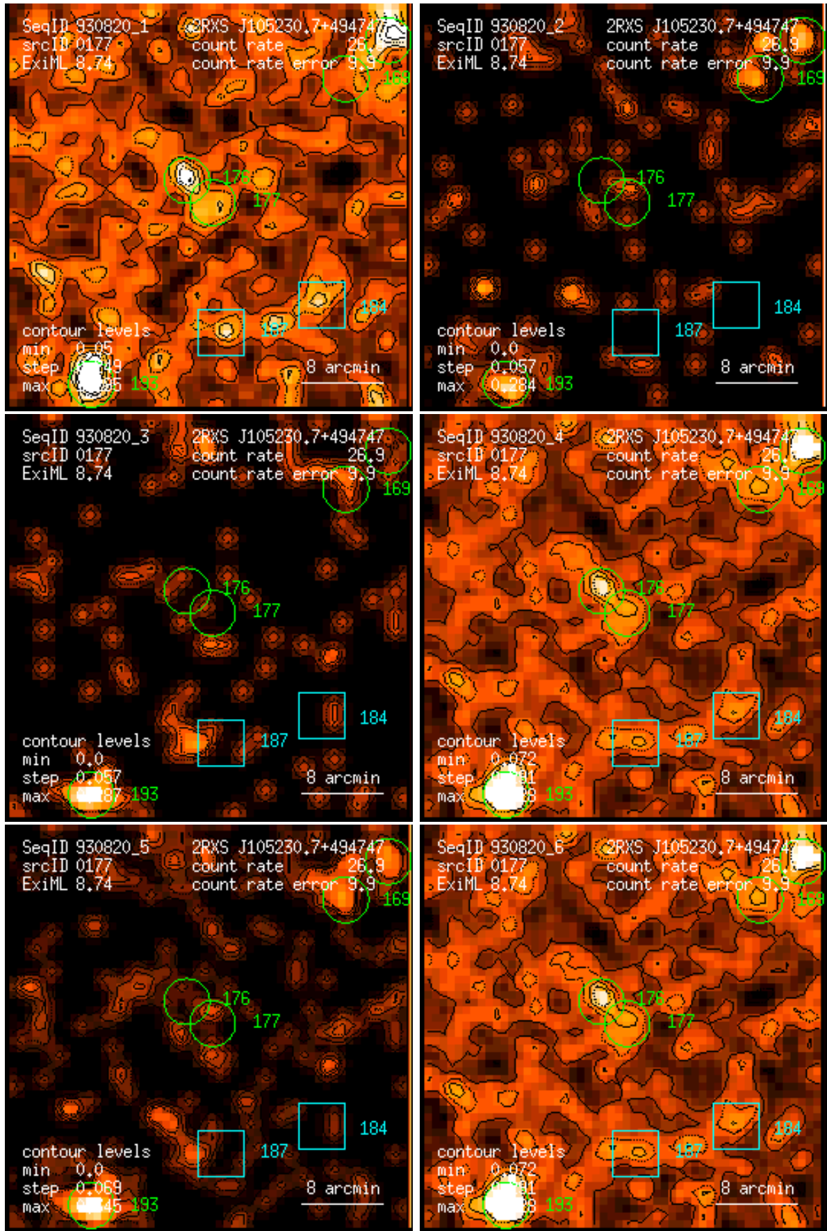
Figure 177: RASS 930820: detection 0177: band rate images, Gaussian filter: (1) PSPC channels 11 – 41, (2) 52 – 90, (3) 91 – 201, (4) 11 – 235, (5) 52 – 201, (6) 11 – 201. Broad band rates in counts/ks. Band rate contour levels in counts/ks/arcmin 2 .
