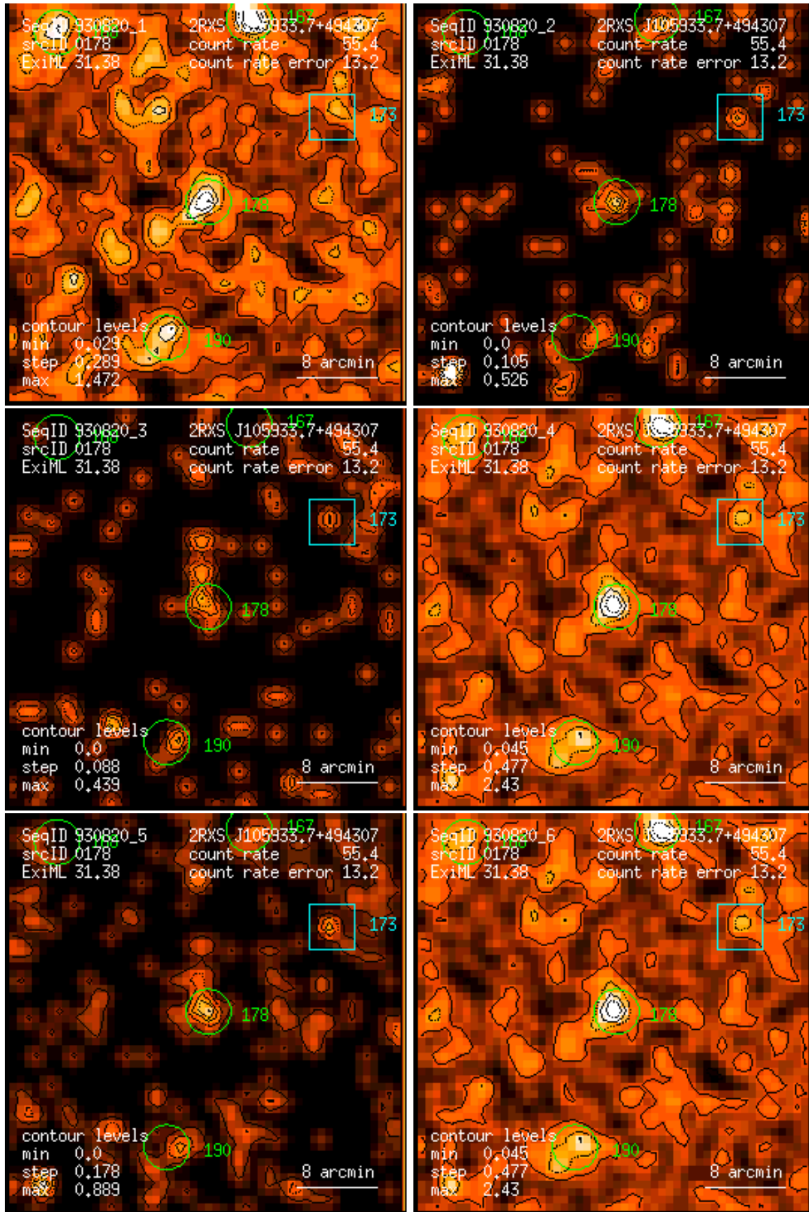
Figure 178: RASS 930820: detection 0178: band rate images, Gaussian filter: (1) PSPC channels 11 – 41, (2) 52 – 90, (3) 91 – 201, (4) 11 – 235, (5) 52 – 201, (6) 11 – 201. Broad band rates in counts/ks. Band rate contour levels in counts/ks/arcmin 2 .
