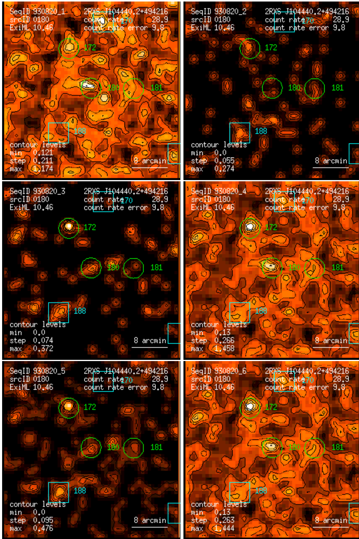
Figure 180: RASS 930820: detection 0180: band rate images, Gaussian filter: (1) PSPC channels 11 – 41, (2) 52 – 90, (3) 91 – 201, (4) 11 – 235, (5) 52 – 201, (6) 11 – 201. Broad band rates in counts/ks. Band rate contour levels in counts/ks/arcmin 2 .
