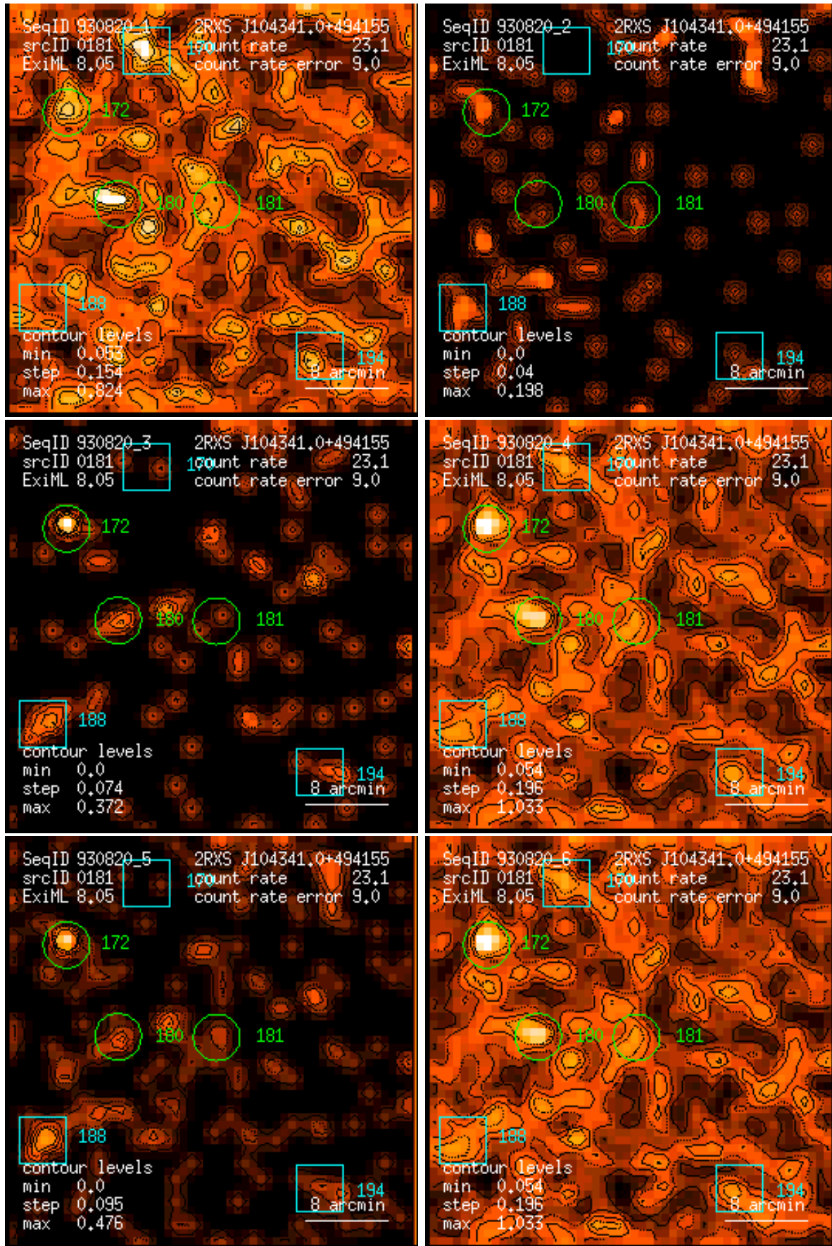
Figure 181: RASS 930820: detection 0181: band rate images, Gaussian filter: (1) PSPC channels 11 – 41, (2) 52 – 90, (3) 91 – 201, (4) 11 – 235, (5) 52 – 201, (6) 11 – 201. Broad band rates in counts/ks. Band rate contour levels in counts/ks/arcmin 2 .
