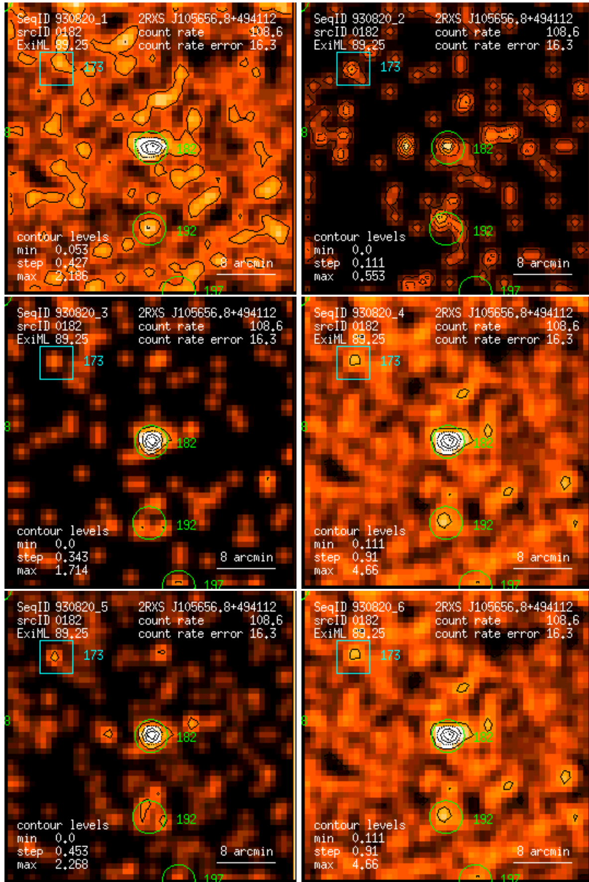
Figure 182: RASS 930820: detection 0182: band rate images, Gaussian filter: (1) PSPC channels 11 – 41, (2) 52 – 90, (3) 91 – 201, (4) 11 – 235, (5) 52 – 201, (6) 11 – 201. Broad band rates in counts/ks. Band rate contour levels in counts/ks/arcmin 2 .
