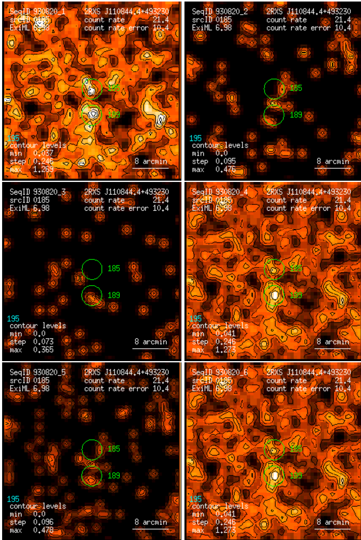
Figure 185: RASS 930820: detection 0185: band rate images, Gaussian filter: (1) PSPC channels 11 – 41, (2) 52 – 90, (3) 91 – 201, (4) 11 – 235, (5) 52 – 201, (6) 11 – 201. Broad band rates in counts/ks. Band rate contour levels in counts/ks/arcmin 2 .
