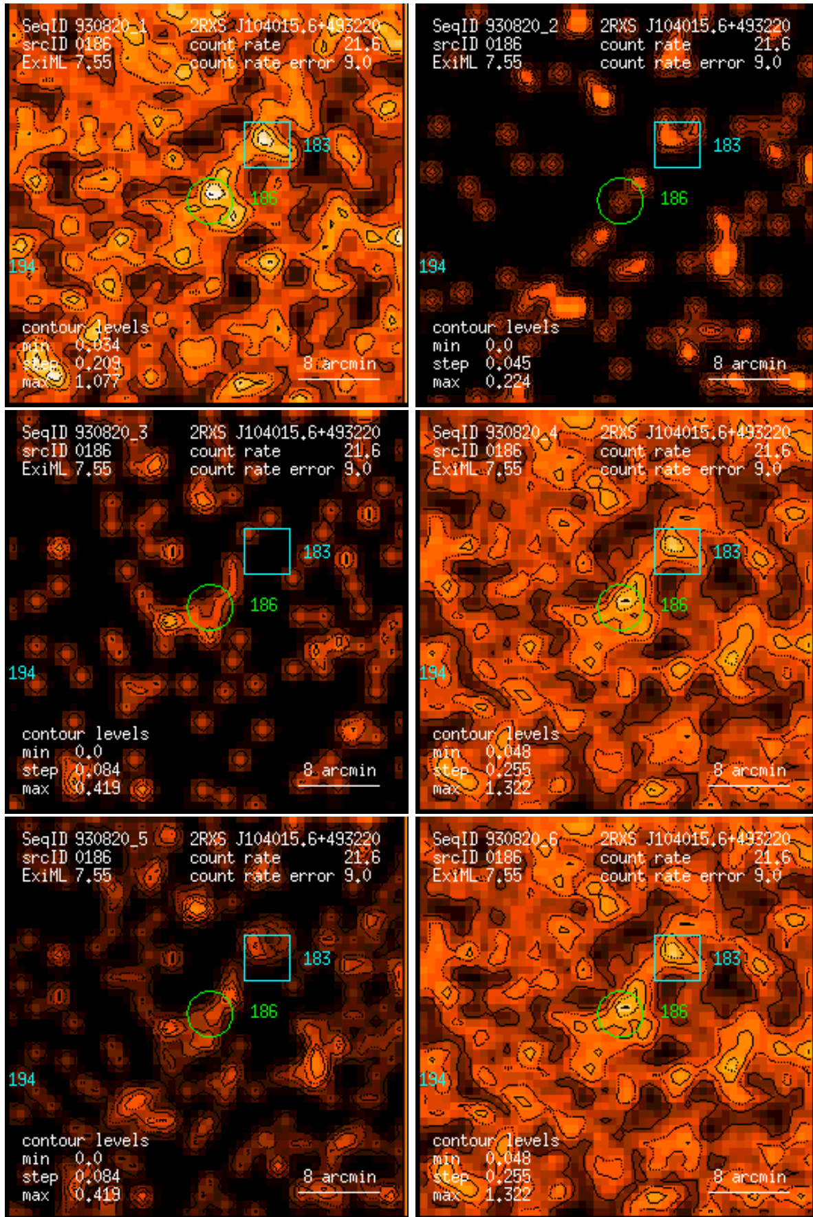
Figure 186: RASS 930820: detection 0186: band rate images, Gaussian filter: (1) PSPC channels 11 – 41, (2) 52 – 90, (3) 91 – 201, (4) 11 – 235, (5) 52 – 201, (6) 11 – 201. Broad band rates in counts/ks. Band rate contour levels in counts/ks/arcmin 2 .
