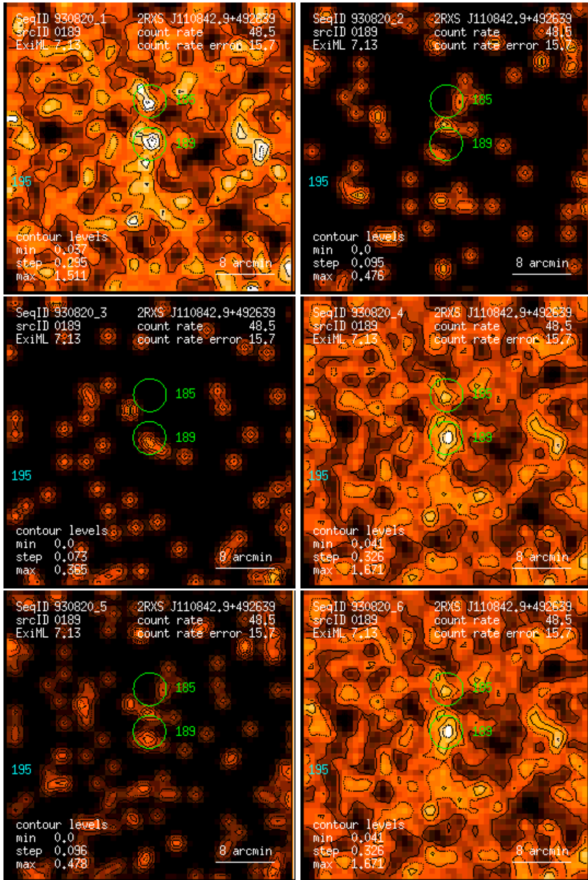
Figure 189: RASS 930820: detection 0189: band rate images, Gaussian filter: (1) PSPC channels 11 – 41, (2) 52 – 90, (3) 91 – 201, (4) 11 – 235, (5) 52 – 201, (6) 11 – 201. Broad band rates in counts/ks. Band rate contour levels in counts/ks/arcmin 2 .
