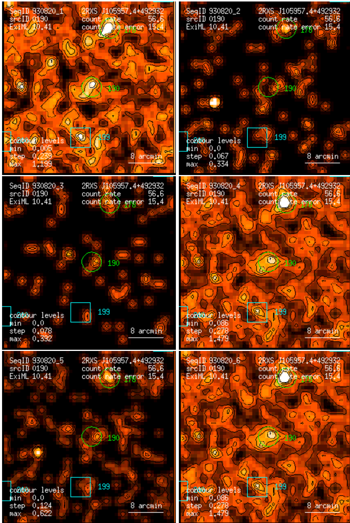
Figure 190: RASS 930820: detection 0190: band rate images, Gaussian filter: (1) PSPC channels 11 – 41, (2) 52 – 90, (3) 91 – 201, (4) 11 – 235, (5) 52 – 201, (6) 11 – 201. Broad band rates in counts/ks. Band rate contour levels in counts/ks/arcmin 2 .
