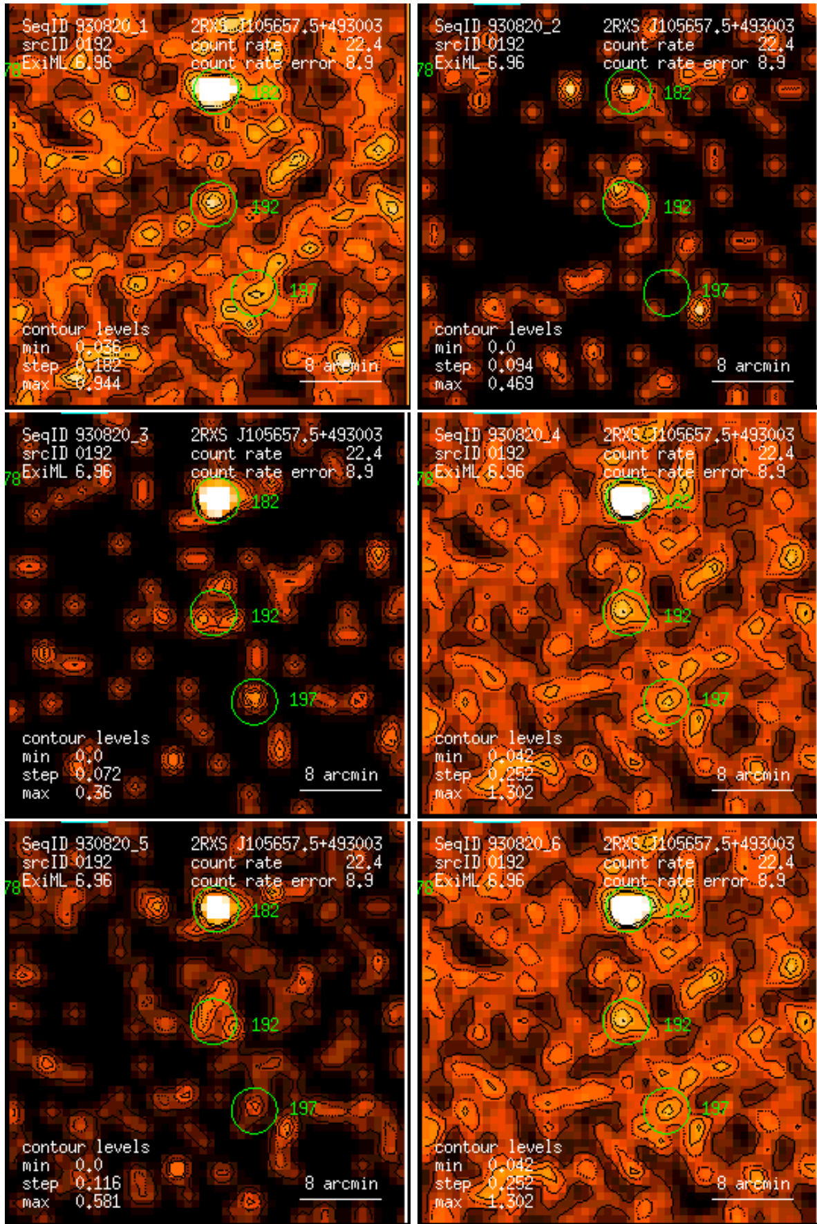
Figure 192: RASS 930820: detection 0192: band rate images, Gaussian filter: (1) PSPC channels 11 – 41, (2) 52 – 90, (3) 91 – 201, (4) 11 – 235, (5) 52 – 201, (6) 11 – 201. Broad band rates in counts/ks. Band rate contour levels in counts/ks/arcmin 2 .
