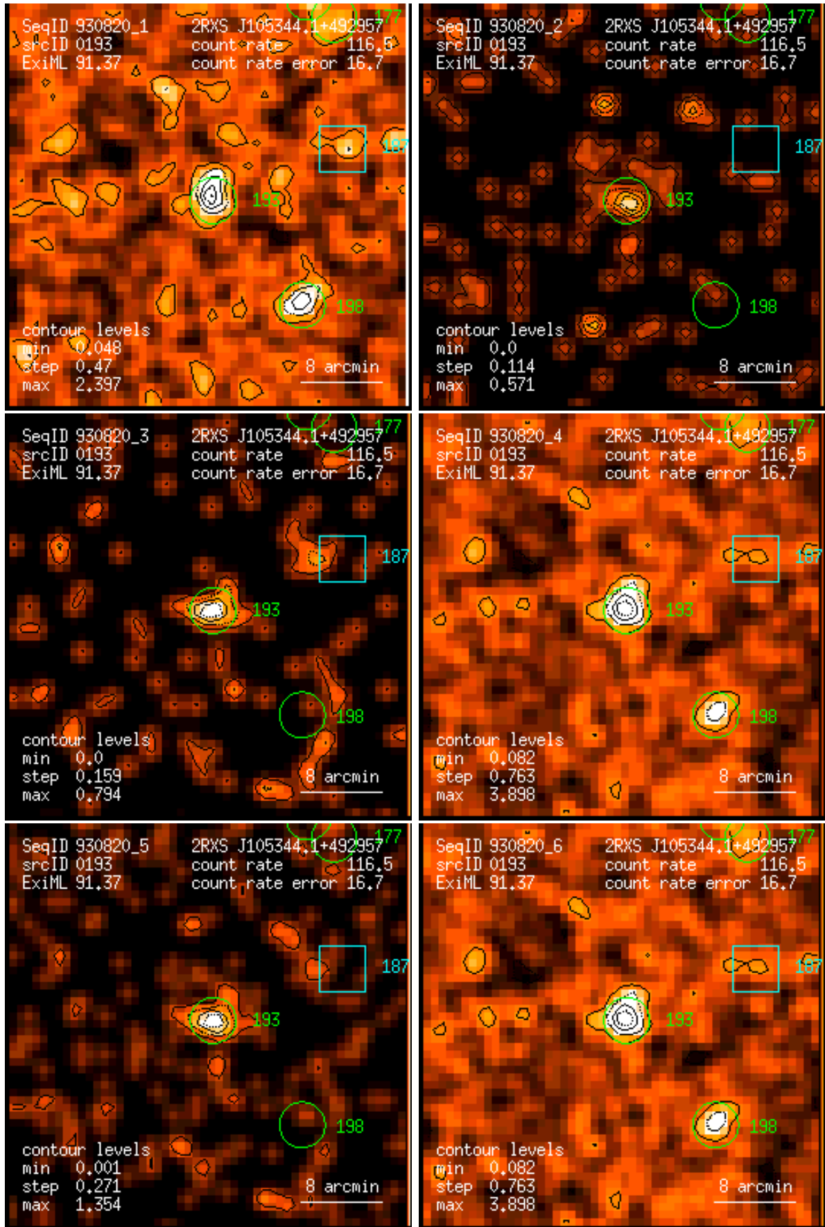
Figure 193: RASS 930820: detection 0193: band rate images, Gaussian filter: (1) PSPC channels 11 – 41, (2) 52 – 90, (3) 91 – 201, (4) 11 – 235, (5) 52 – 201, (6) 11 – 201. Broad band rates in counts/ks. Band rate contour levels in counts/ks/arcmin 2 .
