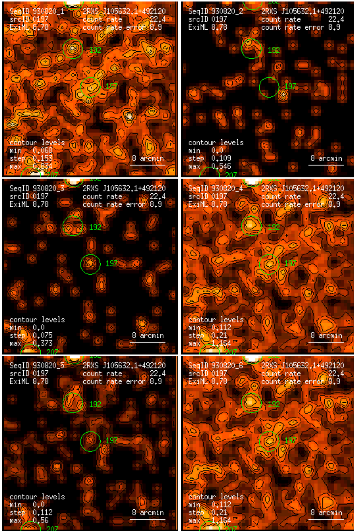
Figure 197: RASS 930820: detection 0197: band rate images, Gaussian filter: (1) PSPC channels 11 – 41, (2) 52 – 90, (3) 91 – 201, (4) 11 – 235, (5) 52 – 201, (6) 11 – 201. Broad band rates in counts/ks. Band rate contour levels in counts/ks/arcmin 2 .
