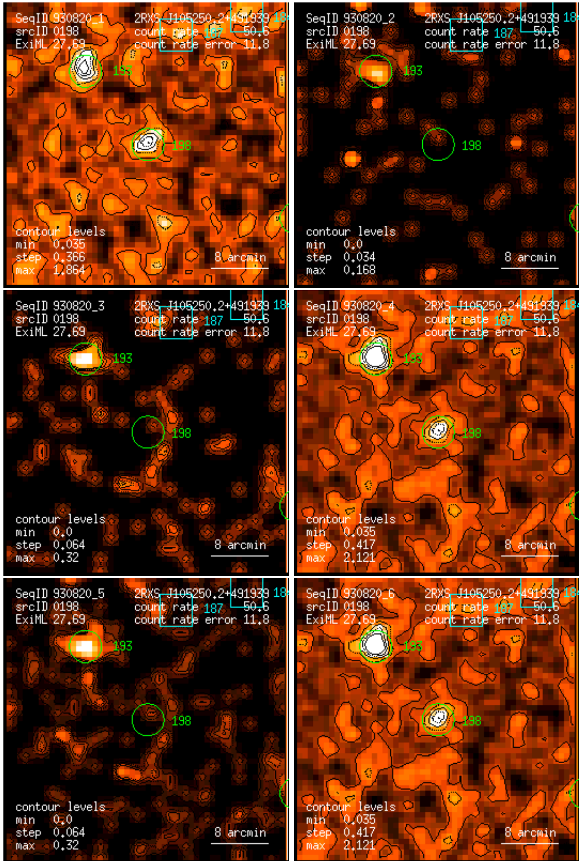
Figure 198: RASS 930820: detection 0198: band rate images, Gaussian filter: (1) PSPC channels 11 – 41, (2) 52 – 90, (3) 91 – 201, (4) 11 – 235, (5) 52 – 201, (6) 11 – 201. Broad band rates in counts/ks. Band rate contour levels in counts/ks/arcmin 2 .
