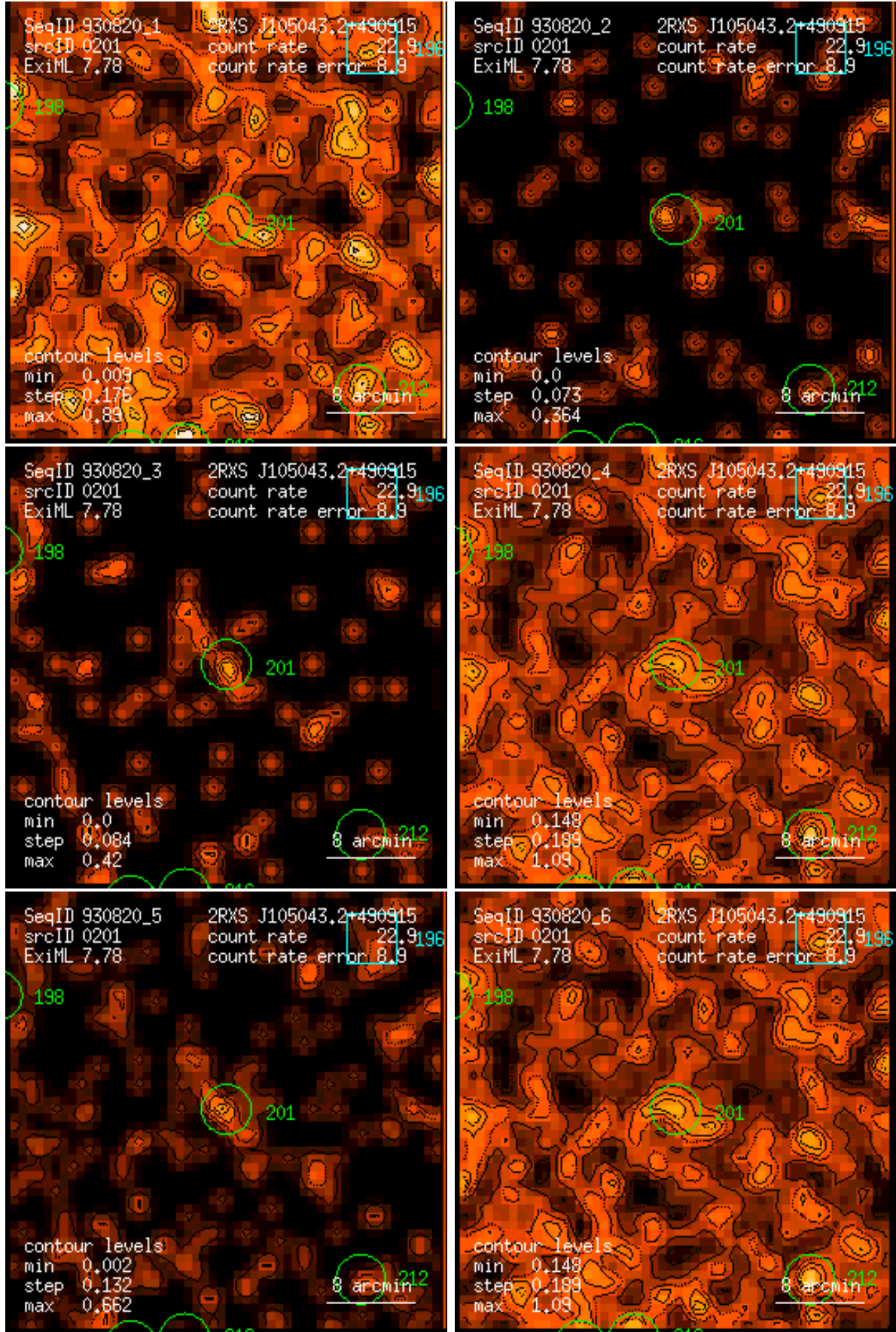
Figure 201: RASS 930820: detection 0201: band rate images, Gaussian filter: (1) PSPC channels 11 – 41, (2) 52 – 90, (3) 91 – 201, (4) 11 – 235, (5) 52 – 201, (6) 11 – 201. Broad band rates in counts/ks. Band rate contour levels in counts/ks/arcmin 2 .
