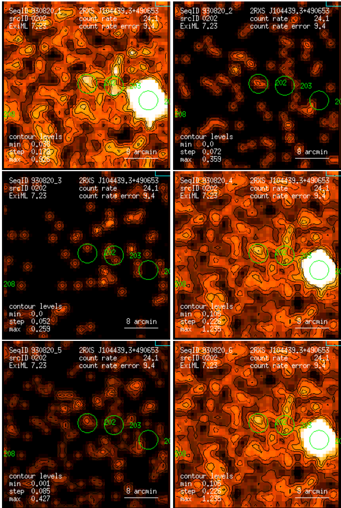
Figure 202: RASS 930820: detection 0202: band rate images, Gaussian filter: (1) PSPC channels 11 – 41, (2) 52 – 90, (3) 91 – 201, (4) 11 – 235, (5) 52 – 201, (6) 11 – 201. Broad band rates in counts/ks. Band rate contour levels in counts/ks/arcmin 2 .
