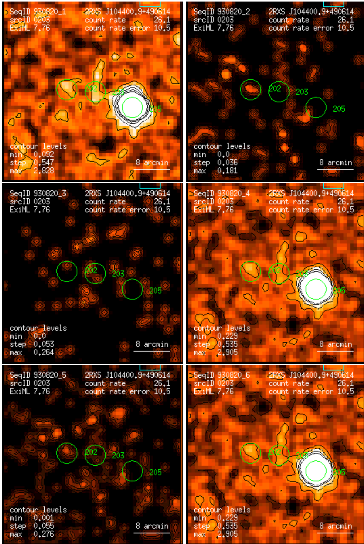
Figure 203: RASS 930820: detection 0203: band rate images, Gaussian filter: (1) PSPC channels 11 – 41, (2) 52 – 90, (3) 91 – 201, (4) 11 – 235, (5) 52 – 201, (6) 11 – 201. Broad band rates in counts/ks. Band rate contour levels in counts/ks/arcmin 2 .
