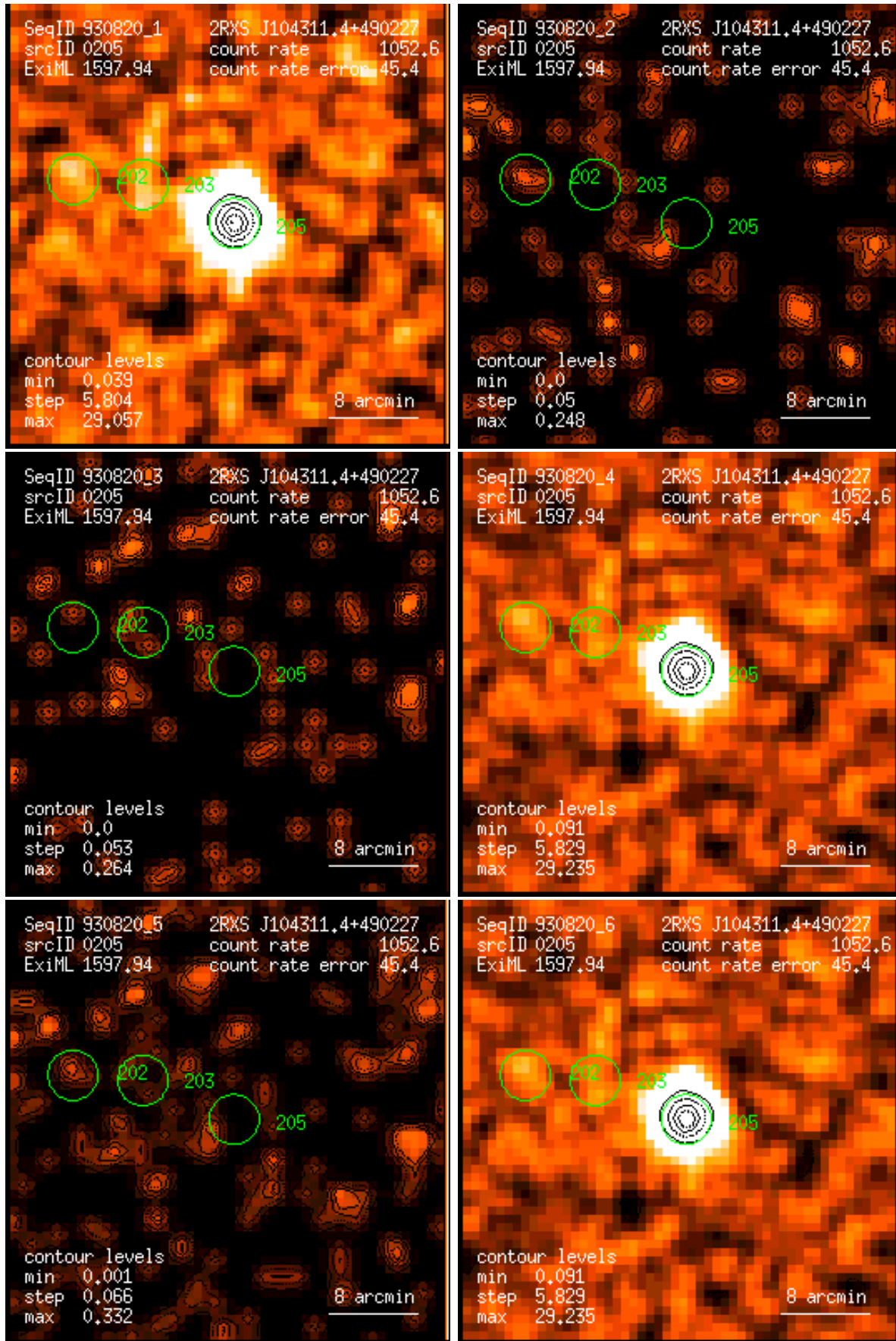
Figure 205: RASS 930820: detection 0205: band rate images, Gaussian filter: (1) PSPC channels 11 – 41, (2) 52 – 90, (3) 91 – 201, (4) 11 – 235, (5) 52 – 201, (6) 11 – 201. Broad band rates in counts/ks. Band rate contour levels in counts/ks/arcmin 2 .
