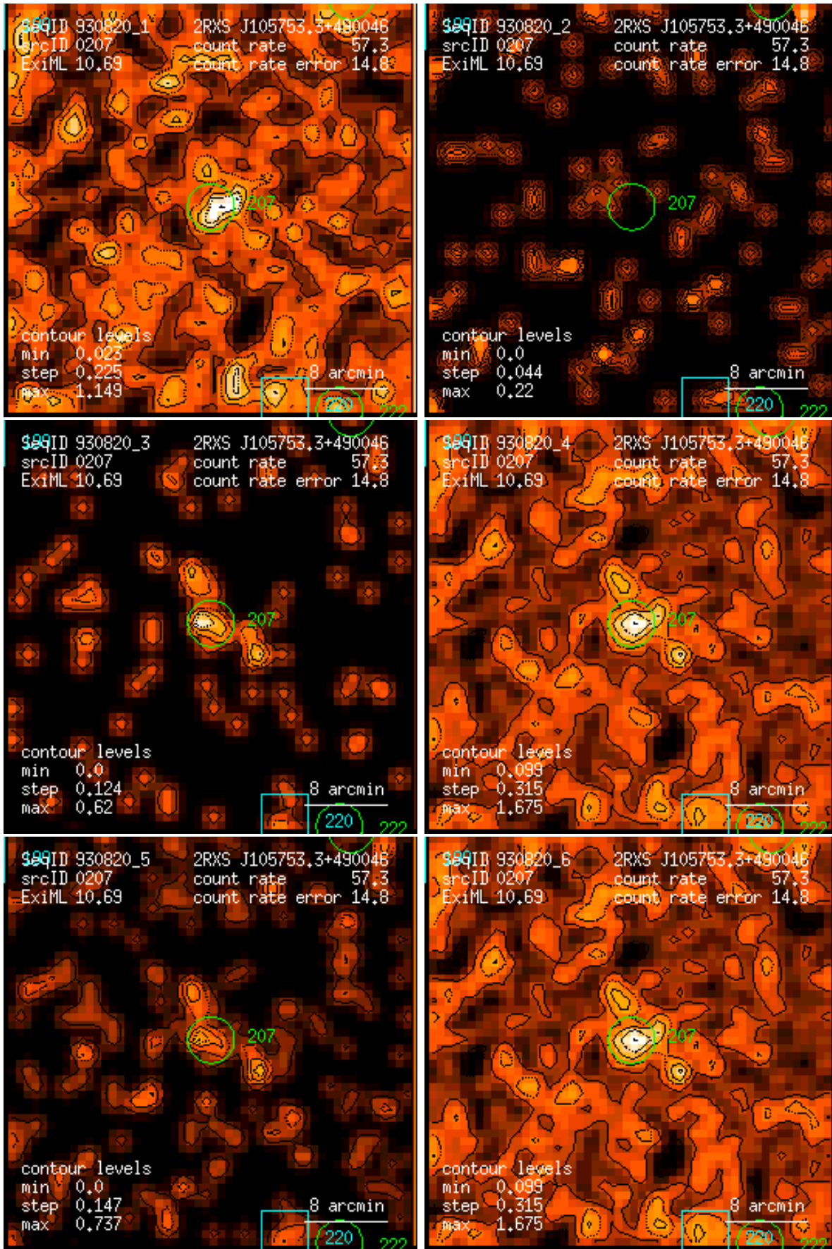
Figure 207: RASS 930820: detection 0207: band rate images, Gaussian filter: (1) PSPC channels 11 – 41, (2) 52 – 90, (3) 91 – 201, (4) 11 – 235, (5) 52 – 201, (6) 11 – 201. Broad band rates in counts/ks. Band rate contour levels in counts/ks/arcmin 2 .
