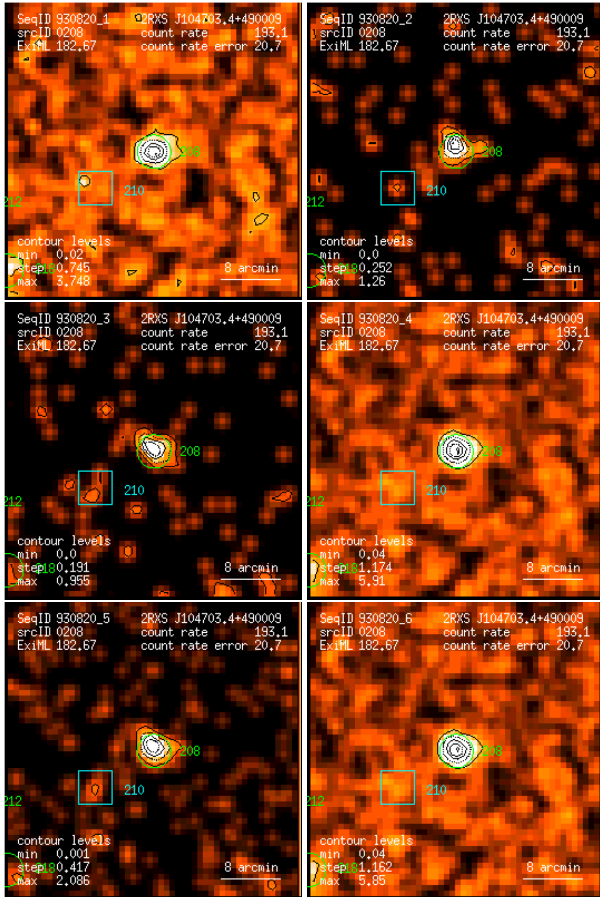
Figure 208: RASS 930820: detection 0208: band rate images, Gaussian filter: (1) PSPC channels 11 – 41, (2) 52 – 90, (3) 91 – 201, (4) 11 – 235, (5) 52 – 201, (6) 11 – 201. Broad band rates in counts/ks. Band rate contour levels in counts/ks/arcmin 2 .
