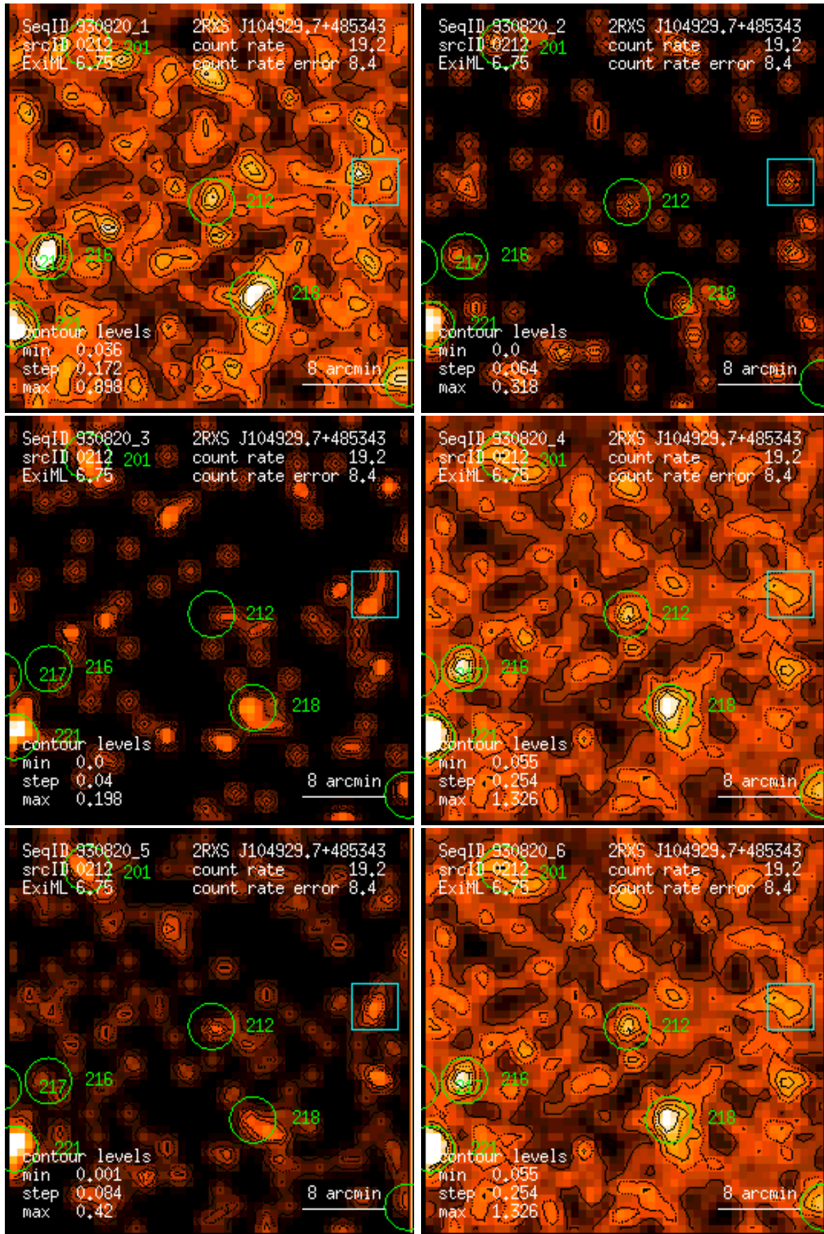
Figure 212: RASS 930820: detection 0212: band rate images, Gaussian filter: (1) PSPC channels 11 – 41, (2) 52 – 90, (3) 91 – 201, (4) 11 – 235, (5) 52 – 201, (6) 11 – 201. Broad band rates in counts/ks. Band rate contour levels in counts/ks/arcmin 2 .
