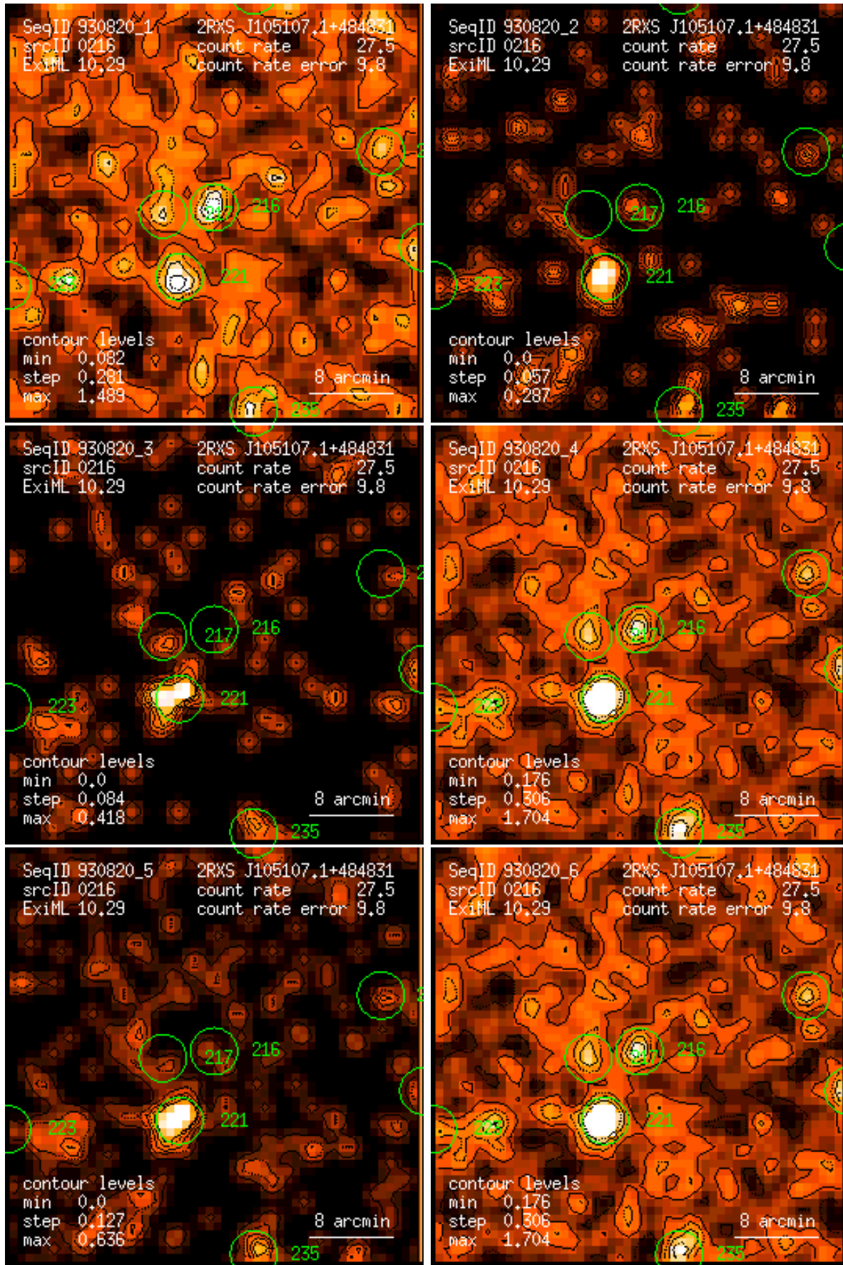
Figure 216: RASS 930820: detection 0216: band rate images, Gaussian filter: (1) PSPC channels 11 – 41, (2) 52 – 90, (3) 91 – 201, (4) 11 – 235, (5) 52 – 201, (6) 11 – 201. Broad band rates in counts/ks. Band rate contour levels in counts/ks/arcmin 2 .
