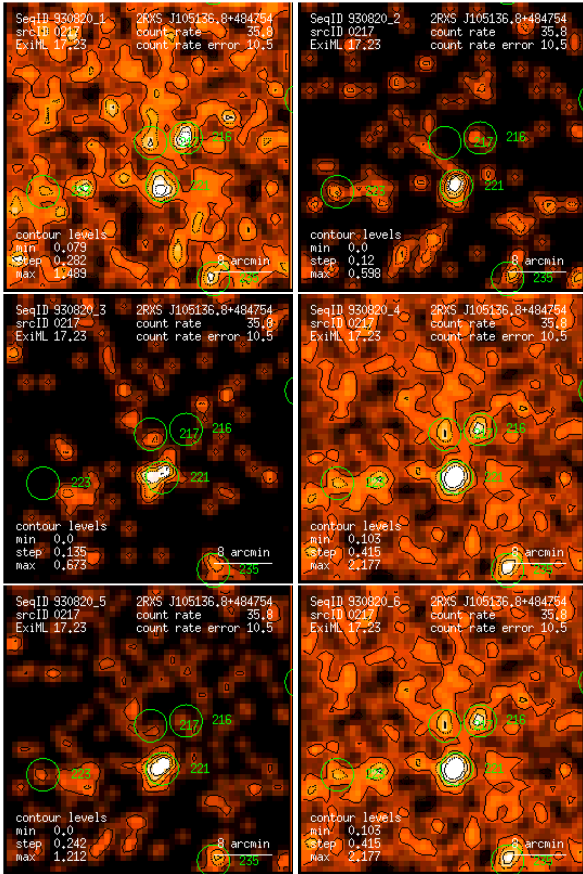
Figure 217: RASS 930820: detection 0217: band rate images, Gaussian filter: (1) PSPC channels 11 – 41, (2) 52 – 90, (3) 91 – 201, (4) 11 – 235, (5) 52 – 201, (6) 11 – 201. Broad band rates in counts/ks. Band rate contour levels in counts/ks/arcmin 2 .
