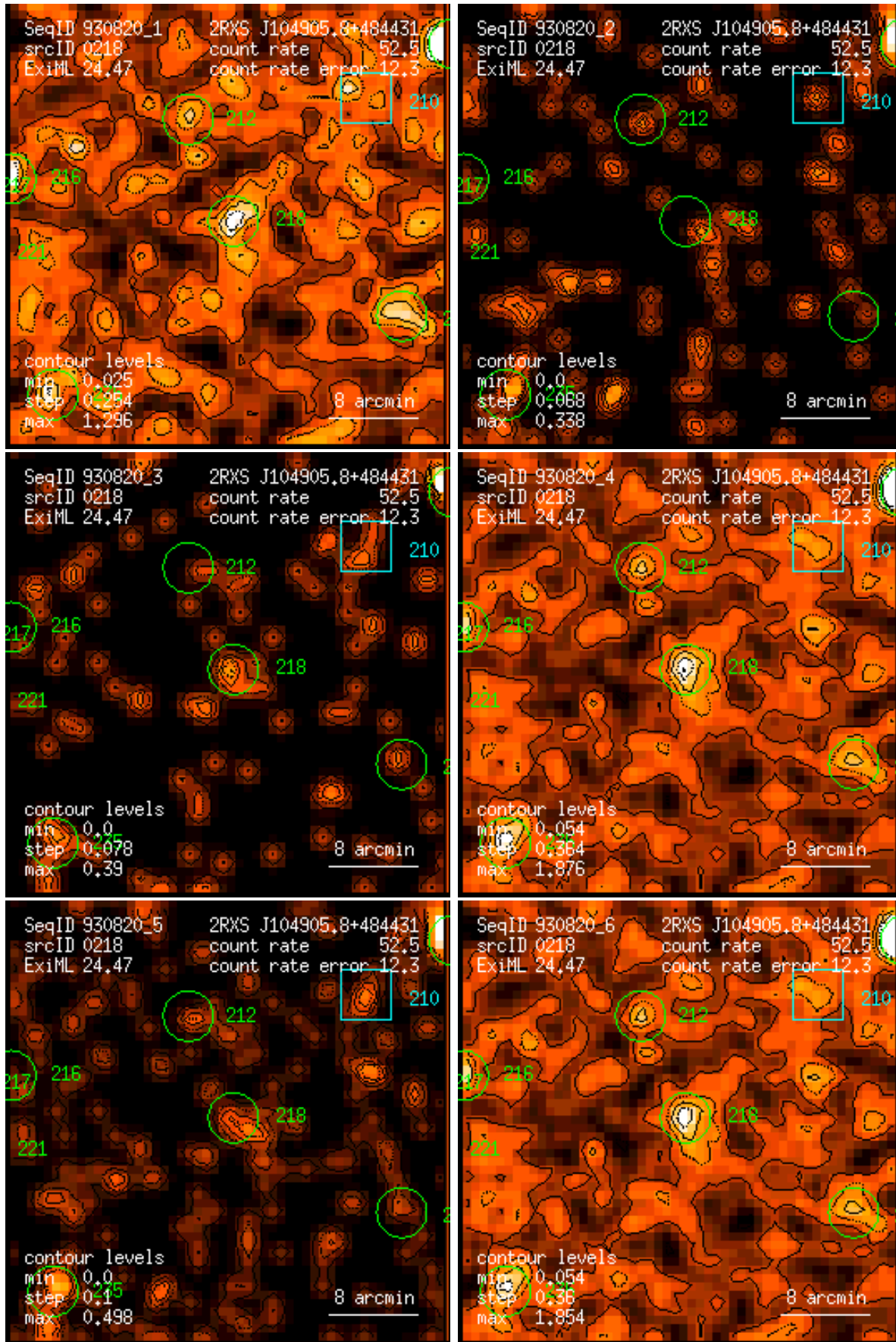
Figure 218: RASS 930820: detection 0218: band rate images, Gaussian filter: (1) PSPC channels 11 – 41, (2) 52 – 90, (3) 91 – 201, (4) 11 – 235, (5) 52 – 201, (6) 11 – 201. Broad band rates in counts/ks. Band rate contour levels in counts/ks/arcmin 2 .
