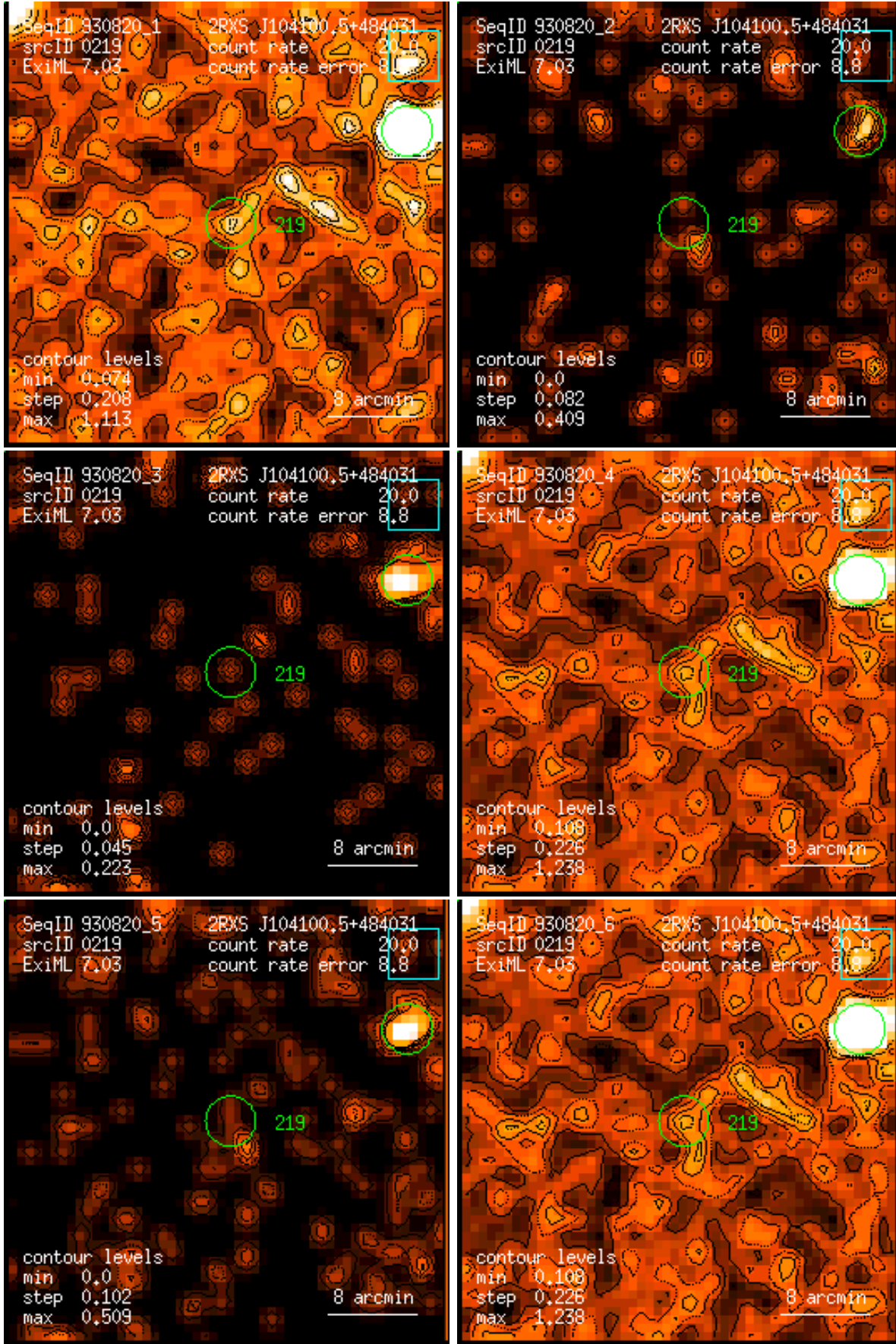
Figure 219: RASS 930820: detection 0219: band rate images, Gaussian filter: (1) PSPC channels 11 – 41, (2) 52 – 90, (3) 91 – 201, (4) 11 – 235, (5) 52 – 201, (6) 11 – 201. Broad band rates in counts/ks. Band rate contour levels in counts/ks/arcmin 2 .
