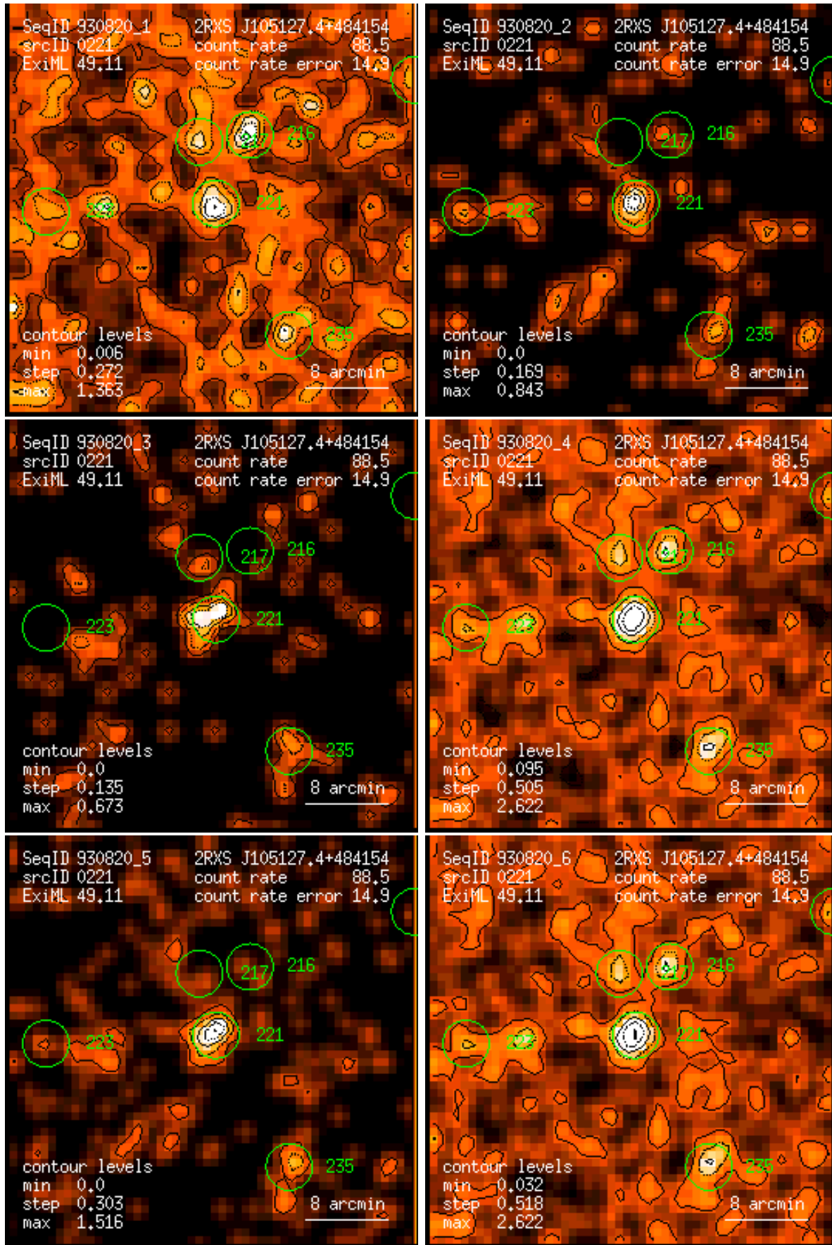
Figure 221: RASS 930820: detection 0221: band rate images, Gaussian filter: (1) PSPC channels 11 – 41, (2) 52 – 90, (3) 91 – 201, (4) 11 – 235, (5) 52 – 201, (6) 11 – 201. Broad band rates in counts/ks. Band rate contour levels in counts/ks/arcmin 2 .
