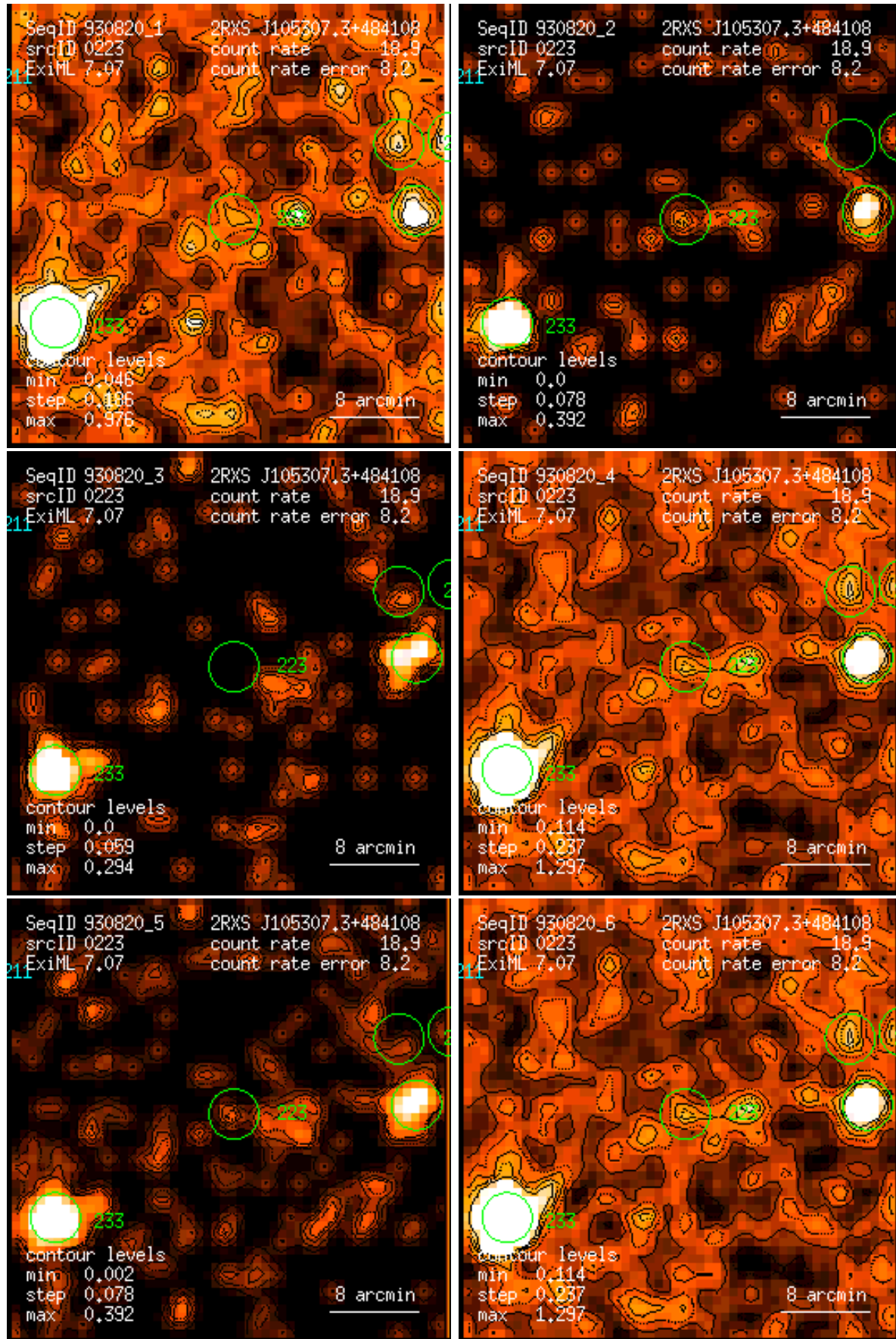
Figure 223: RASS 930820: detection 0223: band rate images, Gaussian filter: (1) PSPC channels 11 – 41, (2) 52 – 90, (3) 91 – 201, (4) 11 – 235, (5) 52 – 201, (6) 11 – 201. Broad band rates in counts/ks. Band rate contour levels in counts/ks/arcmin 2 .
