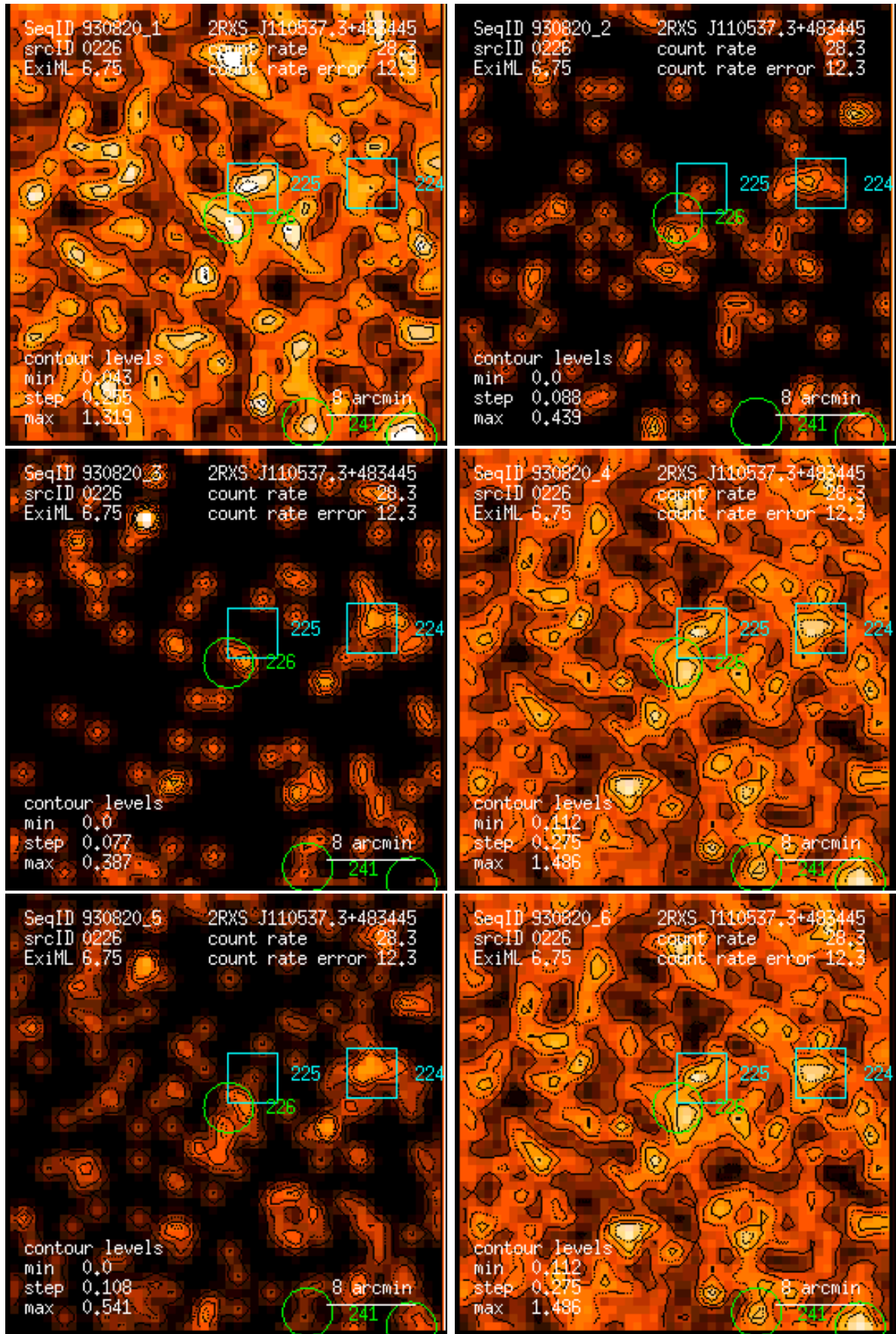
Figure 226: RASS 930820: detection 0226: band rate images, Gaussian filter: (1) PSPC channels 11 – 41, (2) 52 – 90, (3) 91 – 201, (4) 11 – 235, (5) 52 – 201, (6) 11 – 201. Broad band rates in counts/ks. Band rate contour levels in counts/ks/arcmin 2 .
