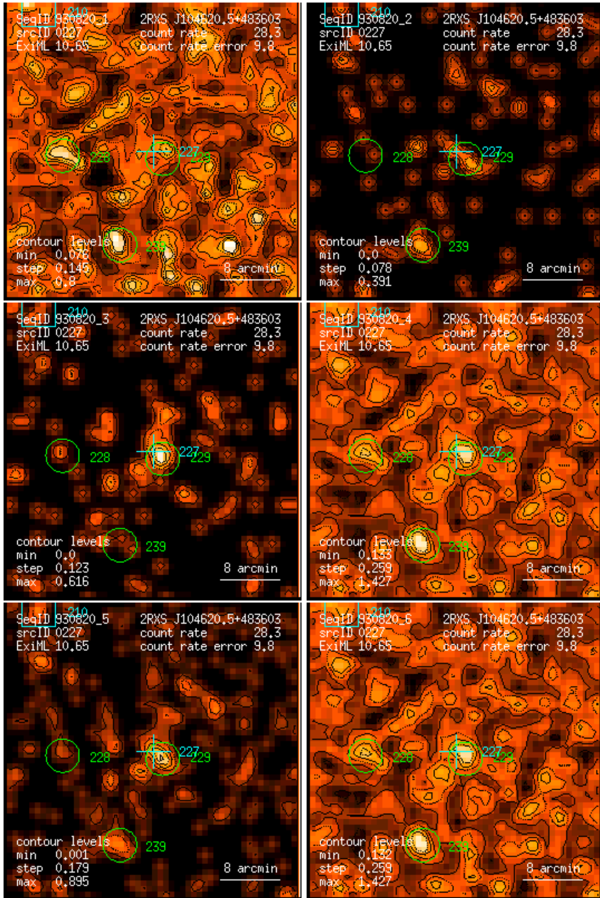
Figure 227: RASS 930820: detection 0227: band rate images, Gaussian filter: (1) PSPC channels 11 – 41, (2) 52 – 90, (3) 91 – 201, (4) 11 – 235, (5) 52 – 201, (6) 11 – 201. Broad band rates in counts/ks. Band rate contour levels in counts/ks/arcmin 2 .
