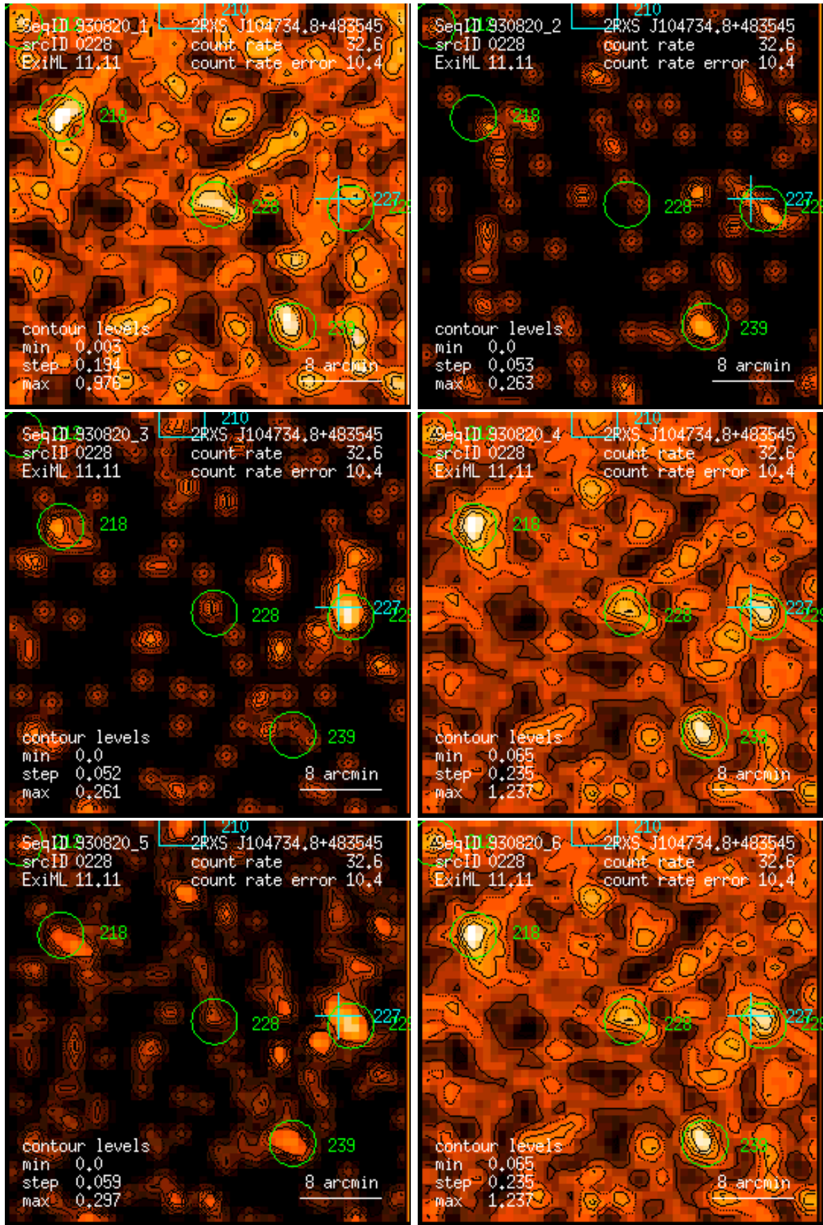
Figure 228: RASS 930820: detection 0228: band rate images, Gaussian filter: (1) PSPC channels 11 – 41, (2) 52 – 90, (3) 91 – 201, (4) 11 – 235, (5) 52 – 201, (6) 11 – 201. Broad band rates in counts/ks. Band rate contour levels in counts/ks/arcmin 2 .
