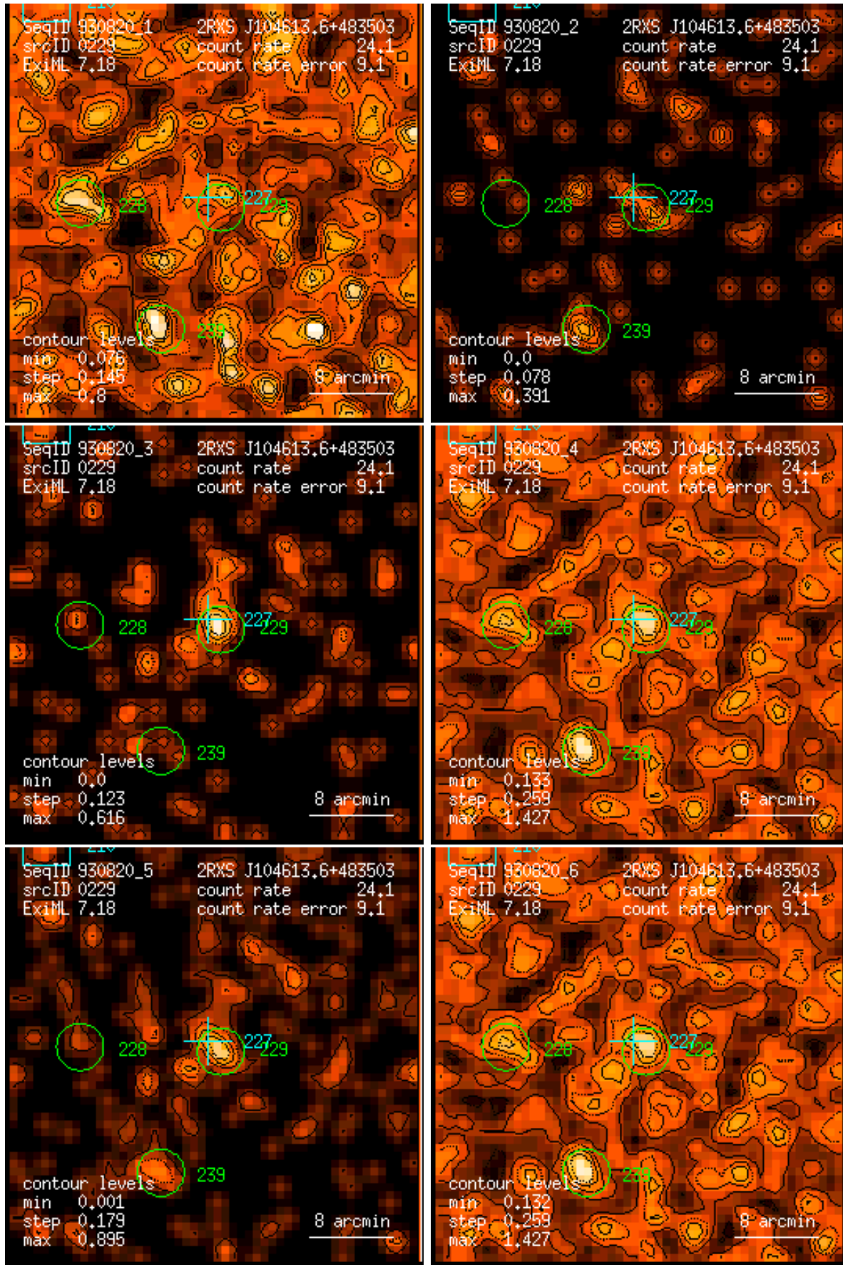
Figure 229: RASS 930820: detection 0229: band rate images, Gaussian filter: (1) PSPC channels 11 – 41, (2) 52 – 90, (3) 91 – 201, (4) 11 – 235, (5) 52 – 201, (6) 11 – 201. Broad band rates in counts/ks. Band rate contour levels in counts/ks/arcmin 2 .
