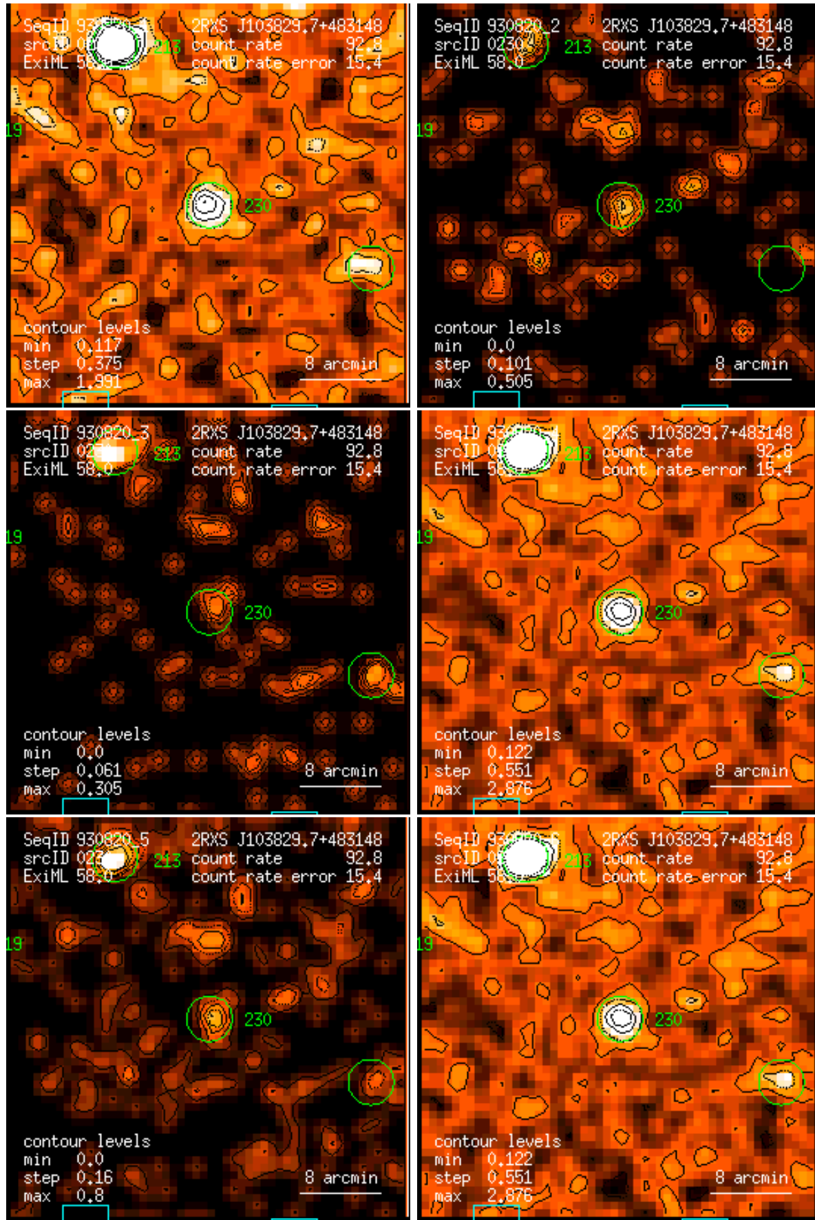
Figure 230: RASS 930820: detection 0230: band rate images, Gaussian filter: (1) PSPC channels 11 – 41, (2) 52 – 90, (3) 91 – 201, (4) 11 – 235, (5) 52 – 201, (6) 11 – 201. Broad band rates in counts/ks. Band rate contour levels in counts/ks/arcmin 2 .
