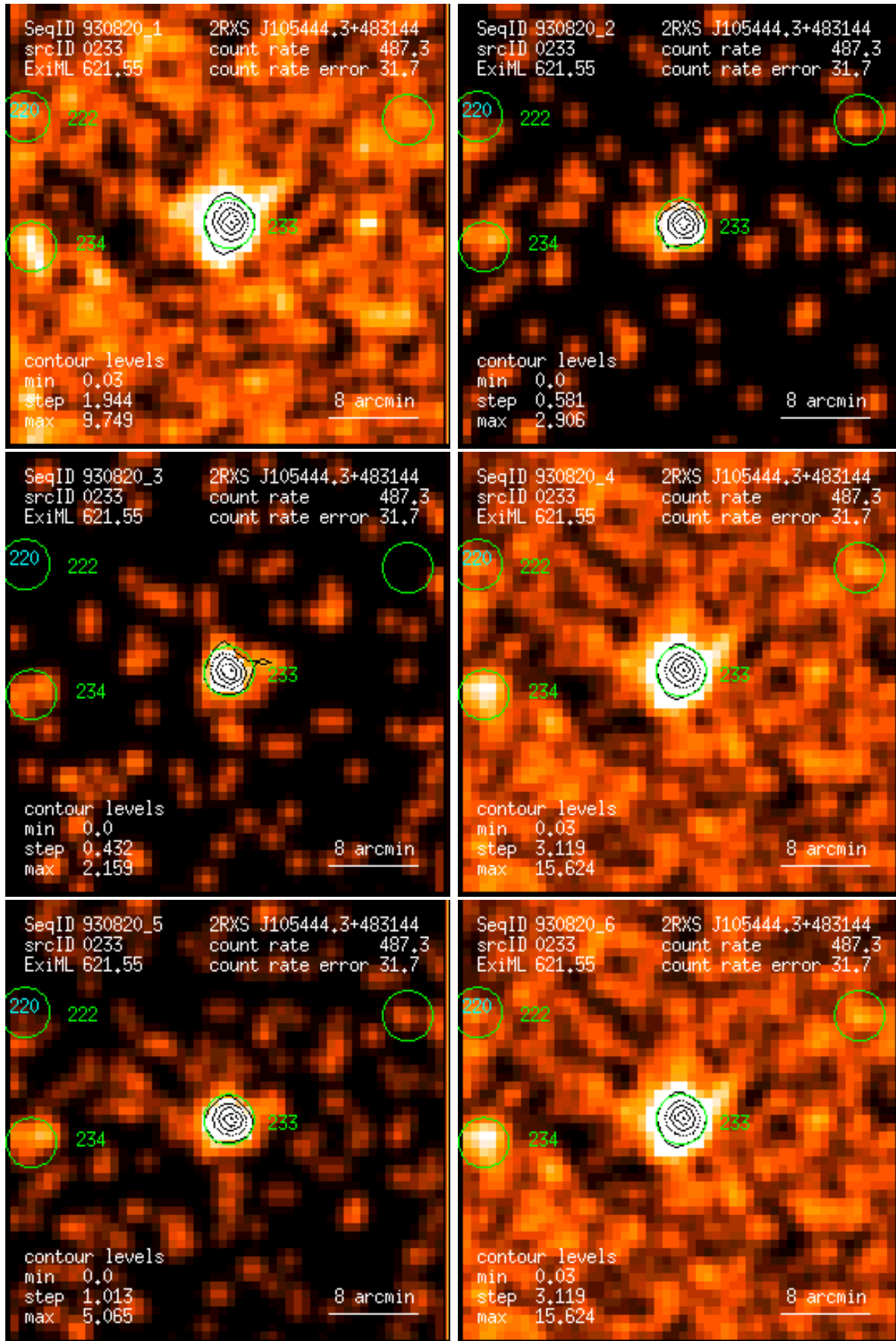
Figure 233: RASS 930820: detection 0233: band rate images, Gaussian filter: (1) PSPC channels 11 – 41, (2) 52 – 90, (3) 91 – 201, (4) 11 – 235, (5) 52 – 201, (6) 11 – 201. Broad band rates in counts/ks. Band rate contour levels in counts/ks/arcmin 2 .
