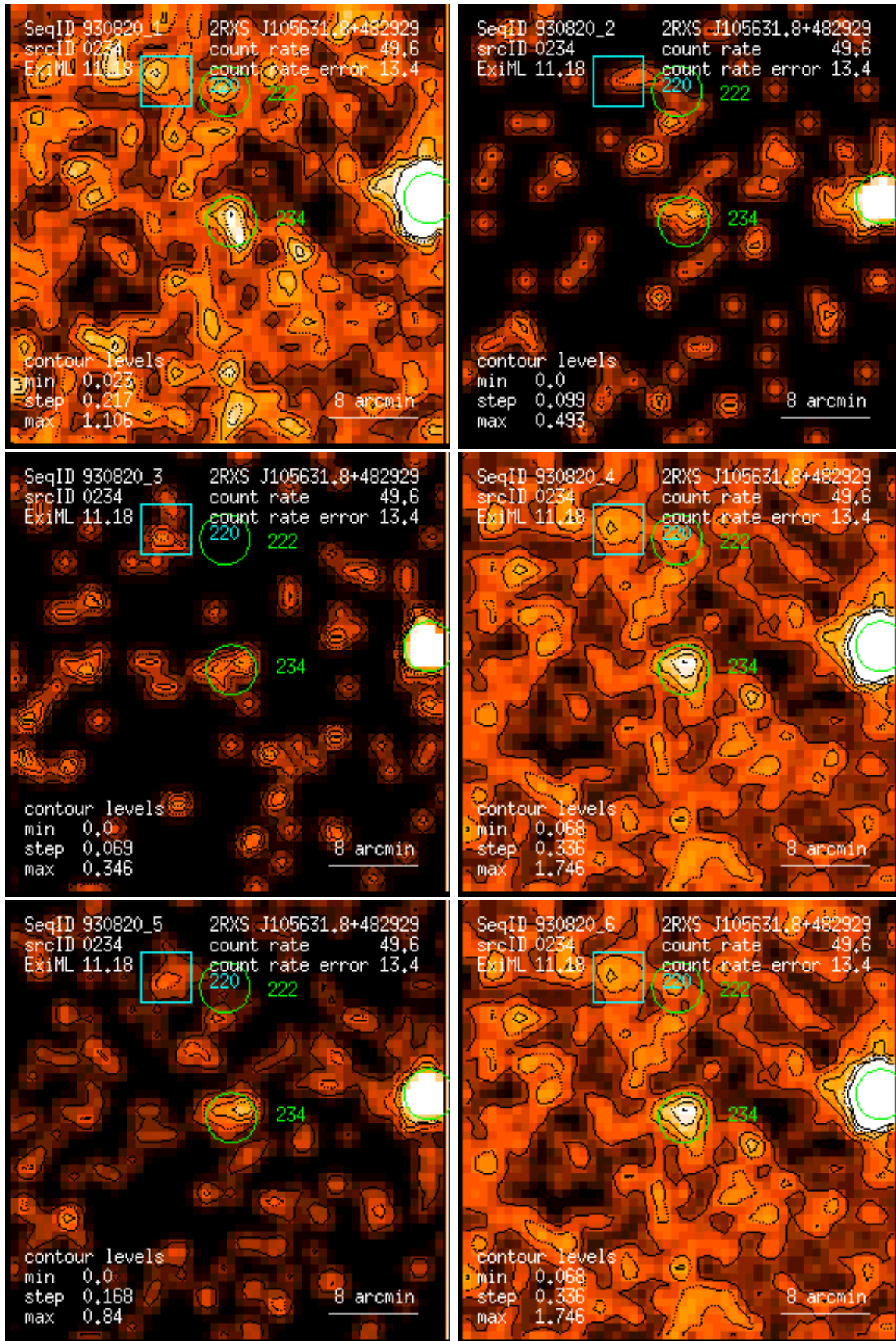
Figure 234: RASS 930820: detection 0234: band rate images, Gaussian filter: (1) PSPC channels 11 – 41, (2) 52 – 90, (3) 91 – 201, (4) 11 – 235, (5) 52 – 201, (6) 11 – 201. Broad band rates in counts/ks. Band rate contour levels in counts/ks/arcmin 2 .
