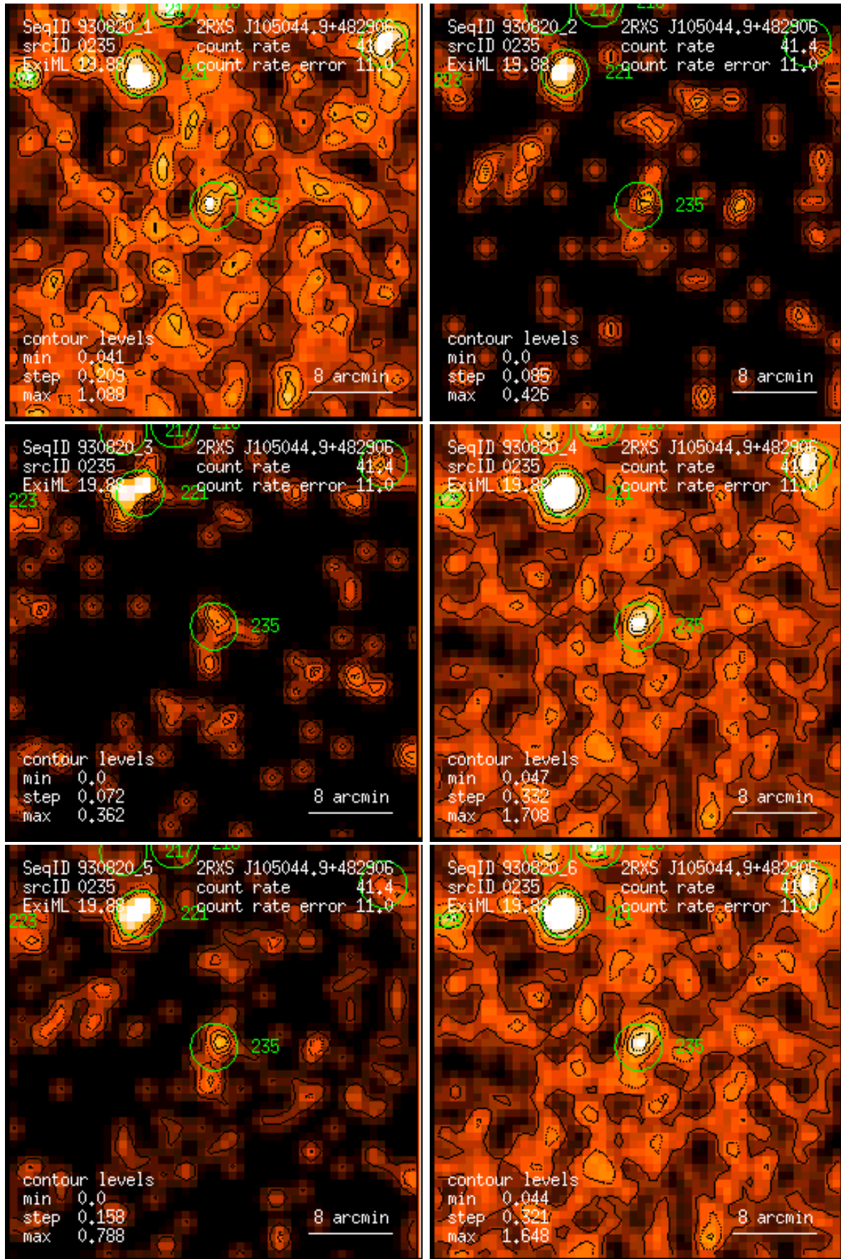
Figure 235: RASS 930820: detection 0235: band rate images, Gaussian filter: (1) PSPC channels 11 – 41, (2) 52 – 90, (3) 91 – 201, (4) 11 – 235, (5) 52 – 201, (6) 11 – 201. Broad band rates in counts/ks. Band rate contour levels in counts/ks/arcmin 2 .
