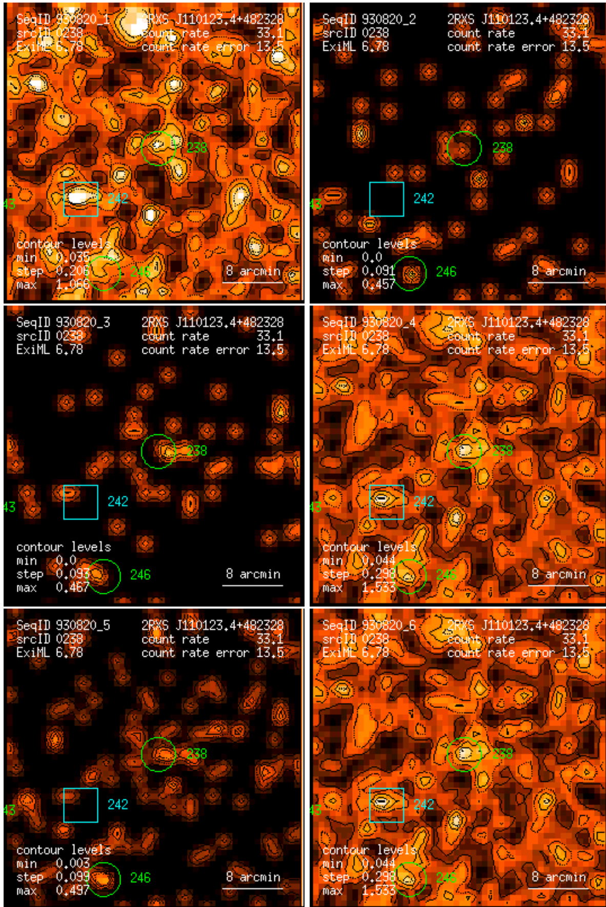
Figure 238: RASS 930820: detection 0238: band rate images, Gaussian filter: (1) PSPC channels 11 – 41, (2) 52 – 90, (3) 91 – 201, (4) 11 – 235, (5) 52 – 201, (6) 11 – 201. Broad band rates in counts/ks. Band rate contour levels in counts/ks/arcmin 2 .
