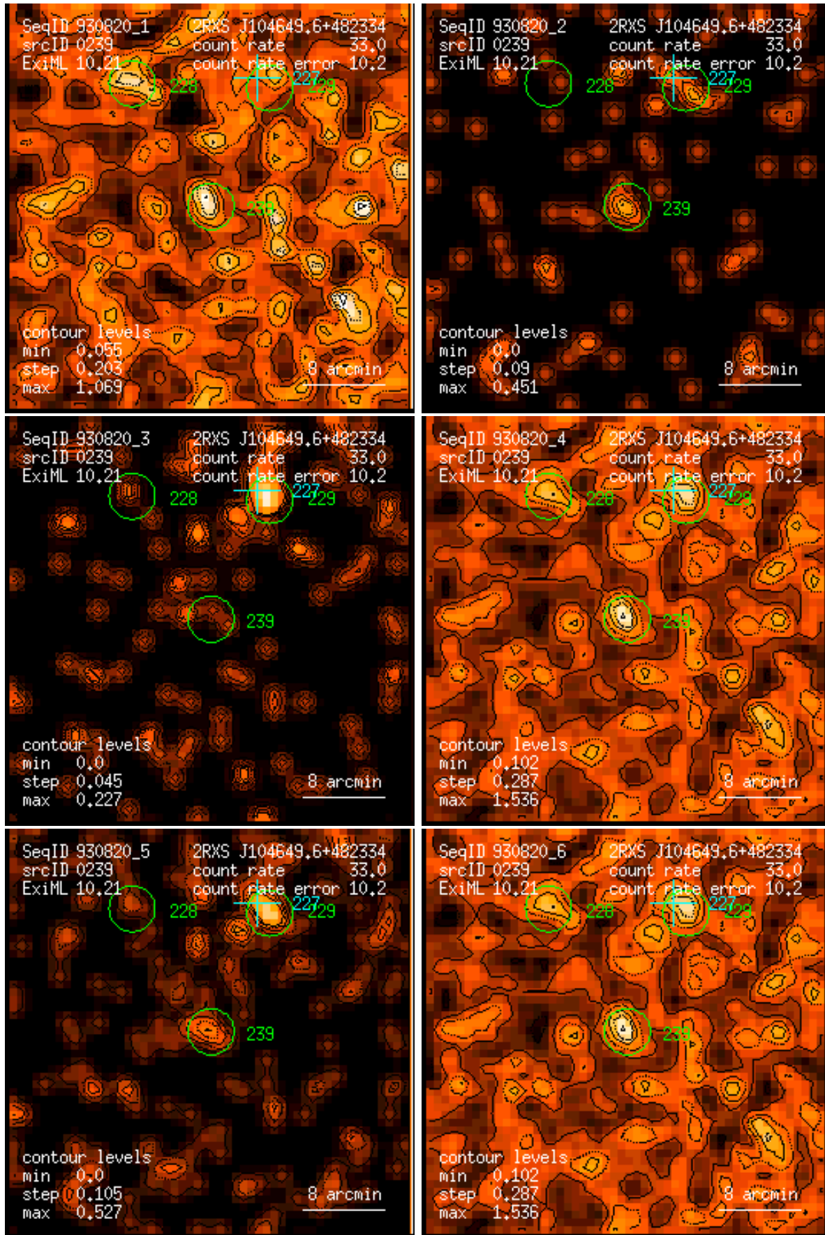
Figure 239: RASS 930820: detection 0239: band rate images, Gaussian filter: (1) PSPC channels 11 – 41, (2) 52 – 90, (3) 91 – 201, (4) 11 – 235, (5) 52 – 201, (6) 11 – 201. Broad band rates in counts/ks. Band rate contour levels in counts/ks/arcmin 2 .
