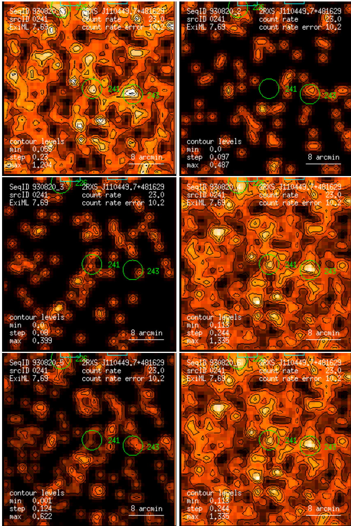
Figure 241: RASS 930820: detection 0241: band rate images, Gaussian filter: (1) PSPC channels 11 – 41, (2) 52 – 90, (3) 91 – 201, (4) 11 – 235, (5) 52 – 201, (6) 11 – 201. Broad band rates in counts/ks. Band rate contour levels in counts/ks/arcmin 2 .
