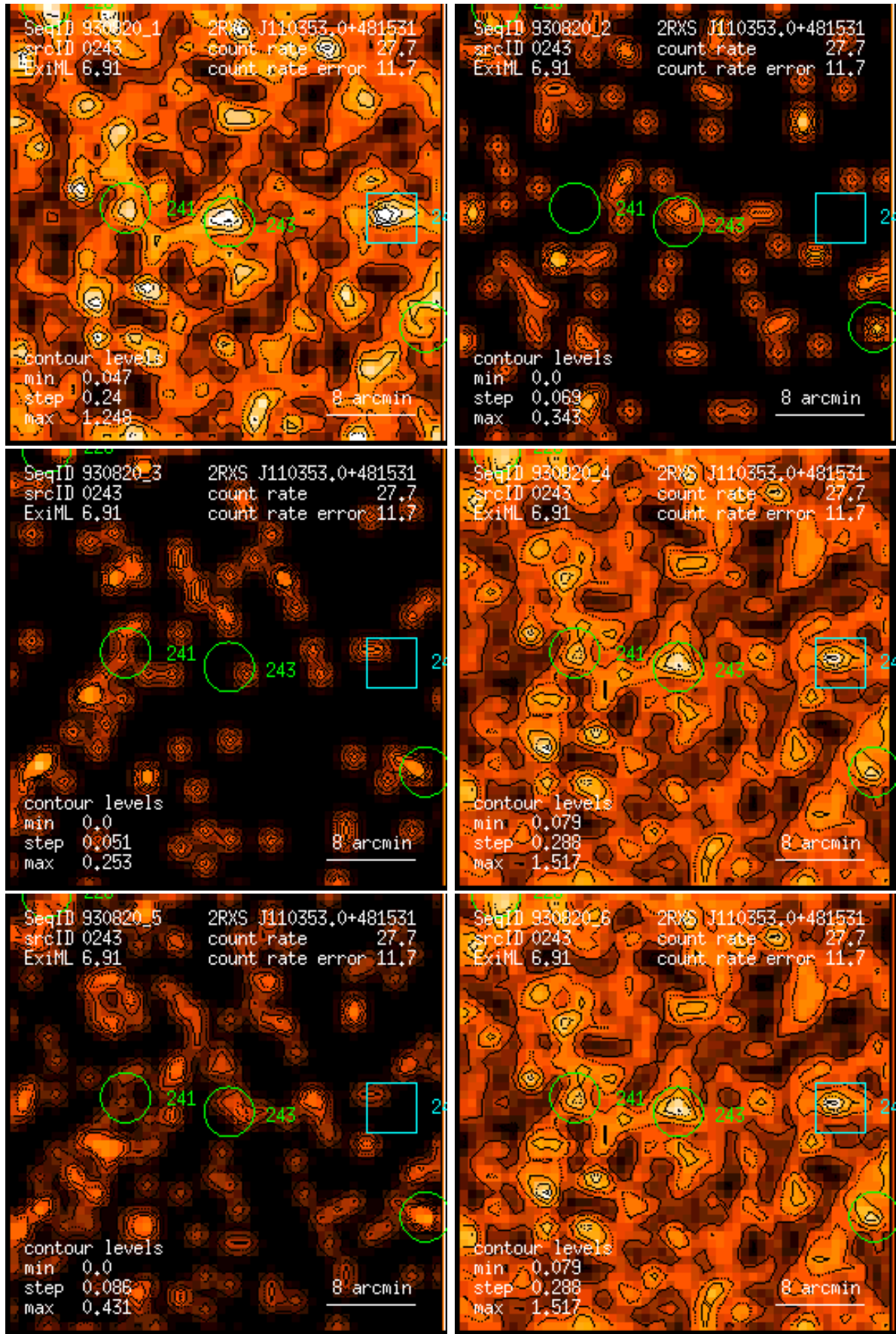
Figure 243: RASS 930820: detection 0243: band rate images, Gaussian filter: (1) PSPC channels 11 – 41, (2) 52 – 90, (3) 91 – 201, (4) 11 – 235, (5) 52 – 201, (6) 11 – 201. Broad band rates in counts/ks. Band rate contour levels in counts/ks/arcmin 2 .
