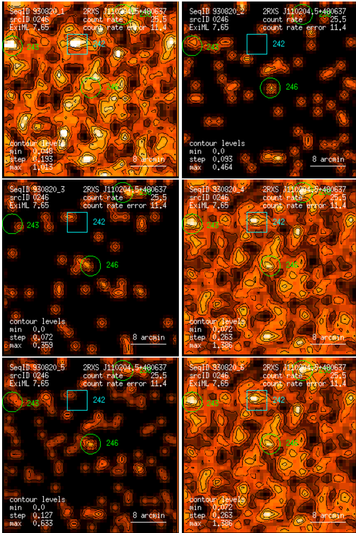
Figure 246: RASS 930820: detection 0246: band rate images, Gaussian filter: (1) PSPC channels 11 – 41, (2) 52 – 90, (3) 91 – 201, (4) 11 – 235, (5) 52 – 201, (6) 11 – 201. Broad band rates in counts/ks. Band rate contour levels in counts/ks/arcmin 2 .
