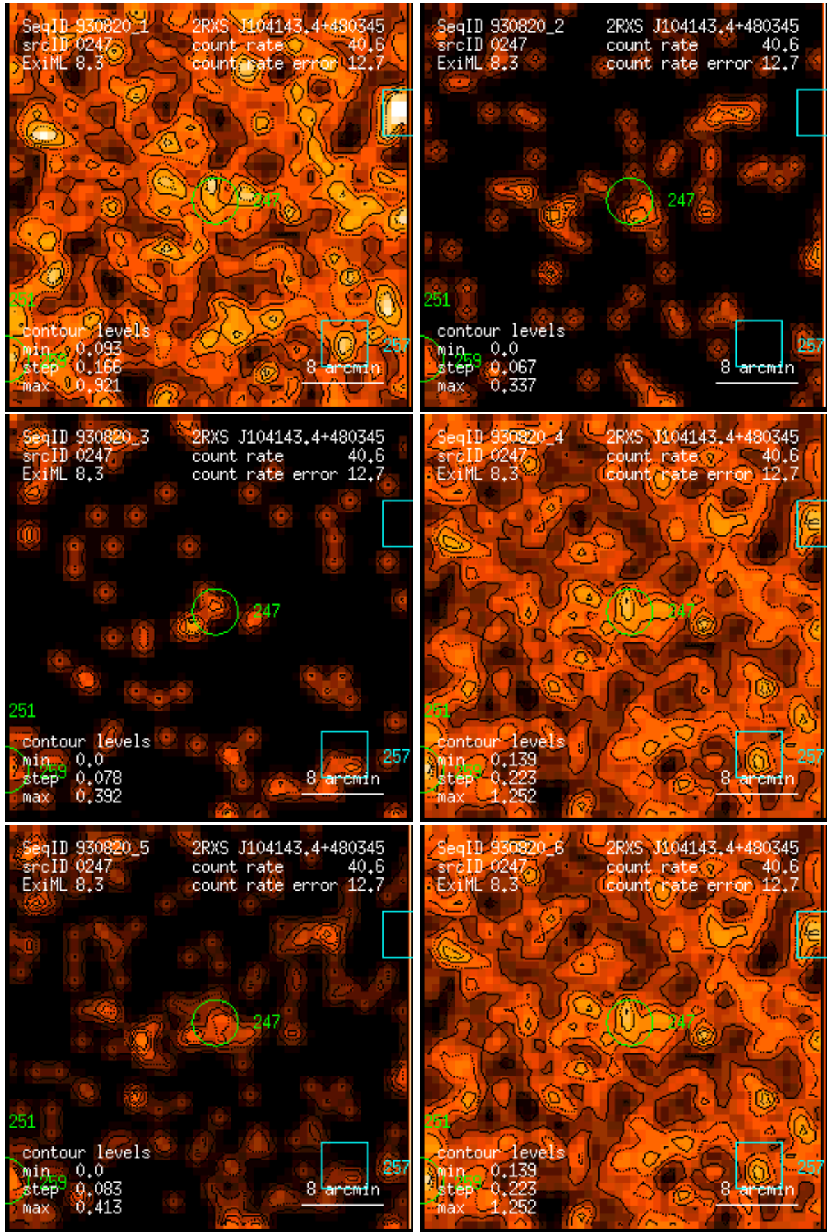
Figure 247: RASS 930820: detection 0247: band rate images, Gaussian filter: (1) PSPC channels 11 – 41, (2) 52 – 90, (3) 91 – 201, (4) 11 – 235, (5) 52 – 201, (6) 11 – 201. Broad band rates in counts/ks. Band rate contour levels in counts/ks/arcmin 2 .
