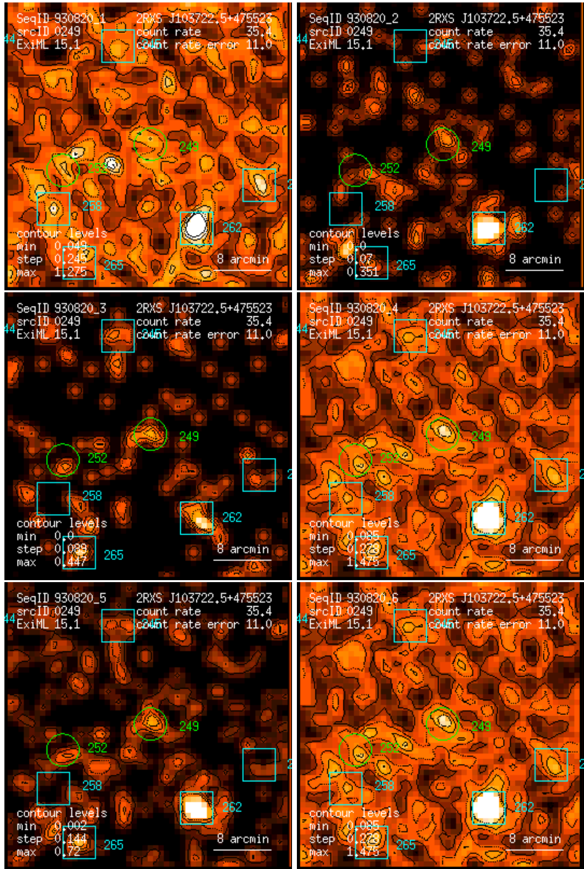
Figure 249: RASS 930820: detection 0249: band rate images, Gaussian filter: (1) PSPC channels 11 – 41, (2) 52 – 90, (3) 91 – 201, (4) 11 – 235, (5) 52 – 201, (6) 11 – 201. Broad band rates in counts/ks. Band rate contour levels in counts/ks/arcmin 2 .
