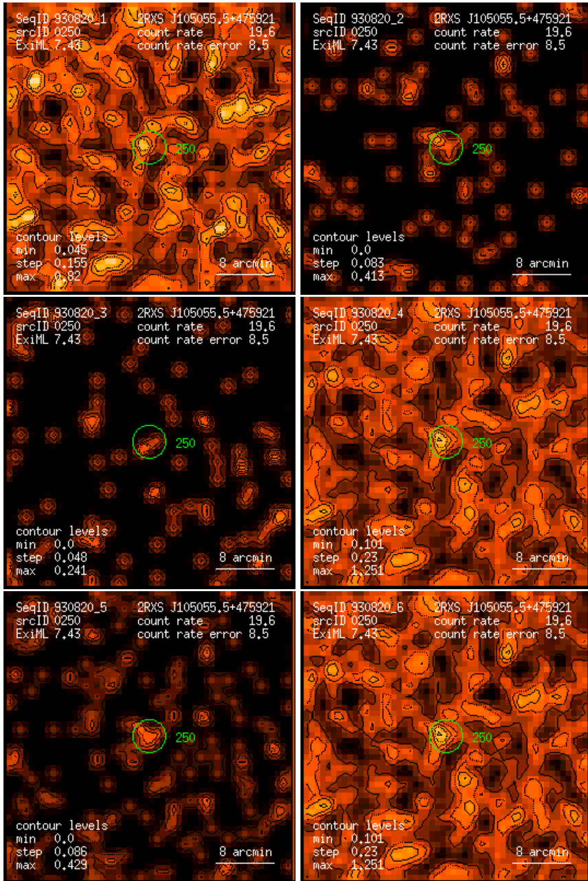
Figure 250: RASS 930820: detection 0250: band rate images, Gaussian filter: (1) PSPC channels 11 – 41, (2) 52 – 90, (3) 91 – 201, (4) 11 – 235, (5) 52 – 201, (6) 11 – 201. Broad band rates in counts/ks. Band rate contour levels in counts/ks/arcmin 2 .
