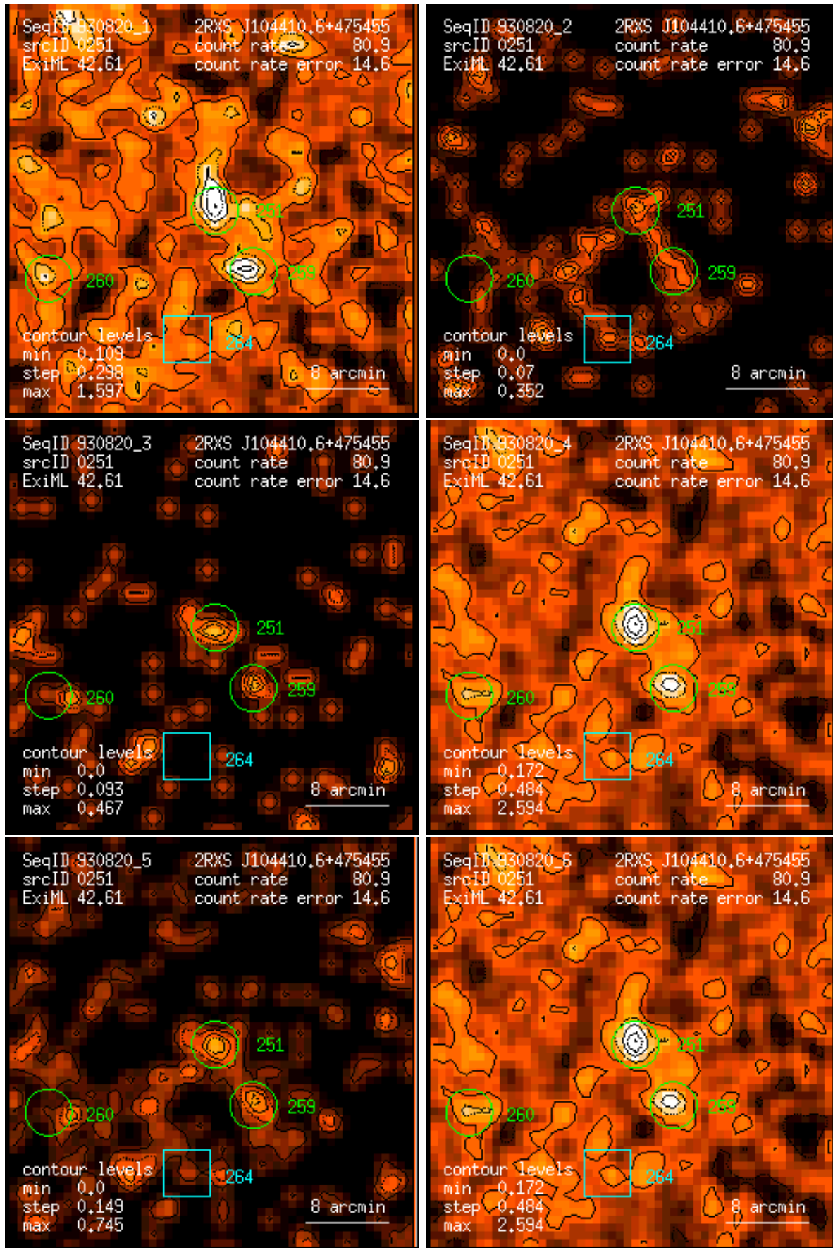
Figure 251: RASS 930820: detection 0251: band rate images, Gaussian filter: (1) PSPC channels 11 – 41, (2) 52 – 90, (3) 91 – 201, (4) 11 – 235, (5) 52 – 201, (6) 11 – 201. Broad band rates in counts/ks. Band rate contour levels in counts/ks/arcmin 2 .
