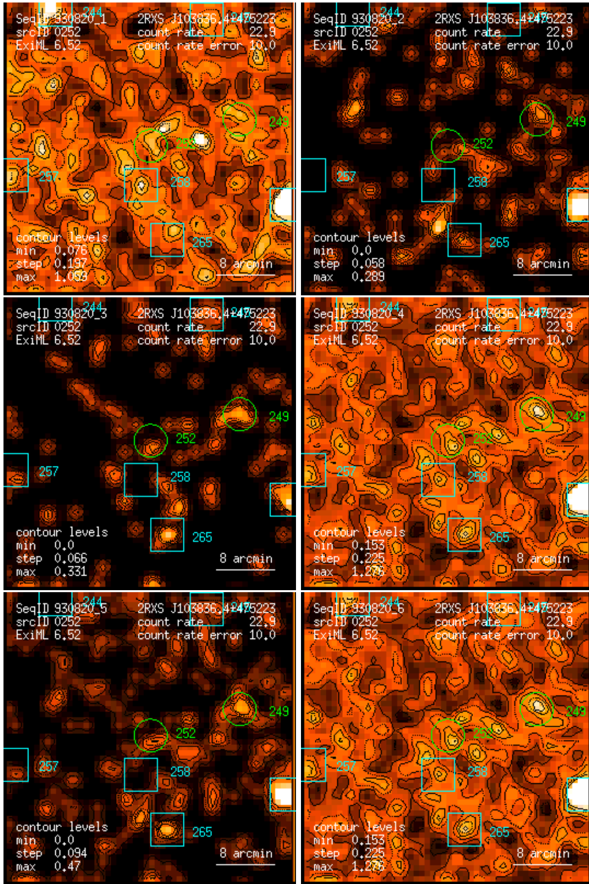
Figure 252: RASS 930820: detection 0252: band rate images, Gaussian filter: (1) PSPC channels 11 – 41, (2) 52 – 90, (3) 91 – 201, (4) 11 – 235, (5) 52 – 201, (6) 11 – 201. Broad band rates in counts/ks. Band rate contour levels in counts/ks/arcmin 2 .
