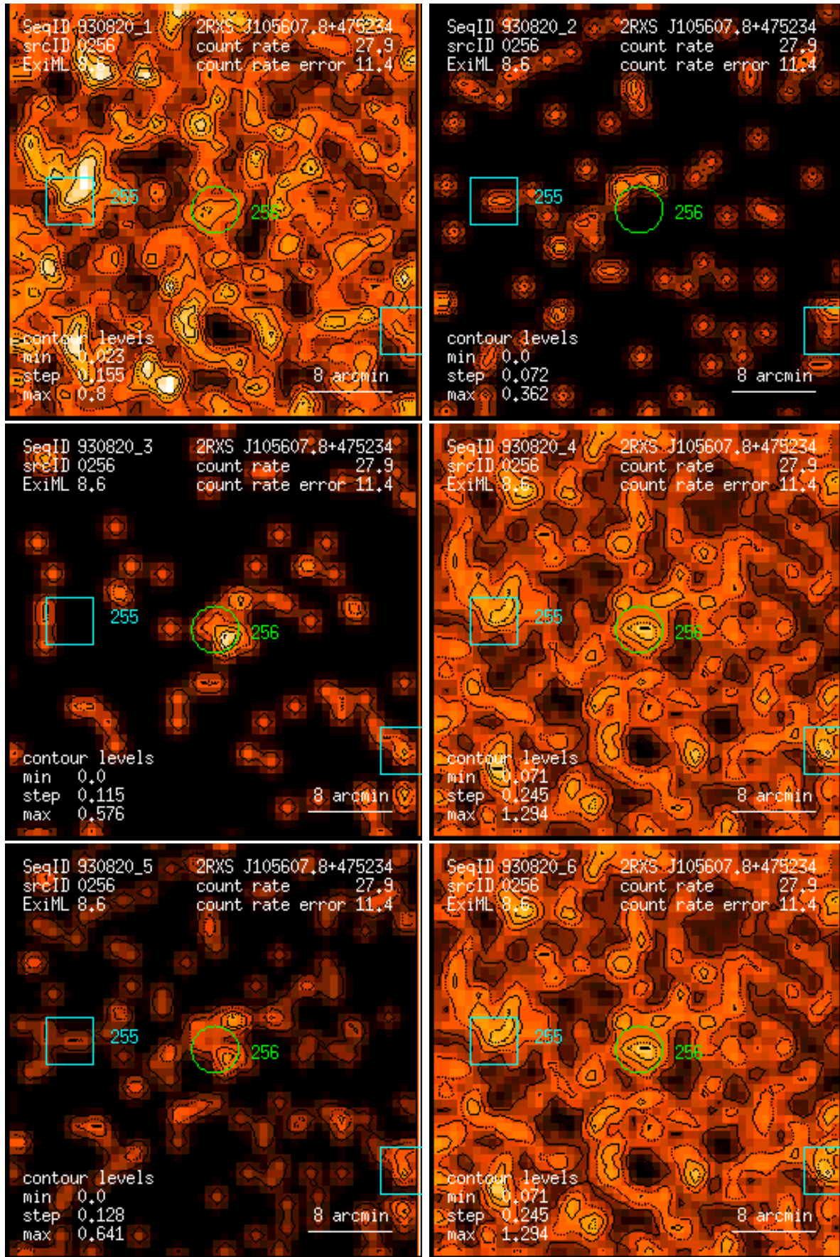
Figure 256: RASS 930820: detection 0256: band rate images, Gaussian filter: (1) PSPC channels 11 – 41, (2) 52 – 90, (3) 91 – 201, (4) 11 – 235, (5) 52 – 201, (6) 11 – 201. Broad band rates in counts/ks. Band rate contour levels in counts/ks/arcmin 2 .
