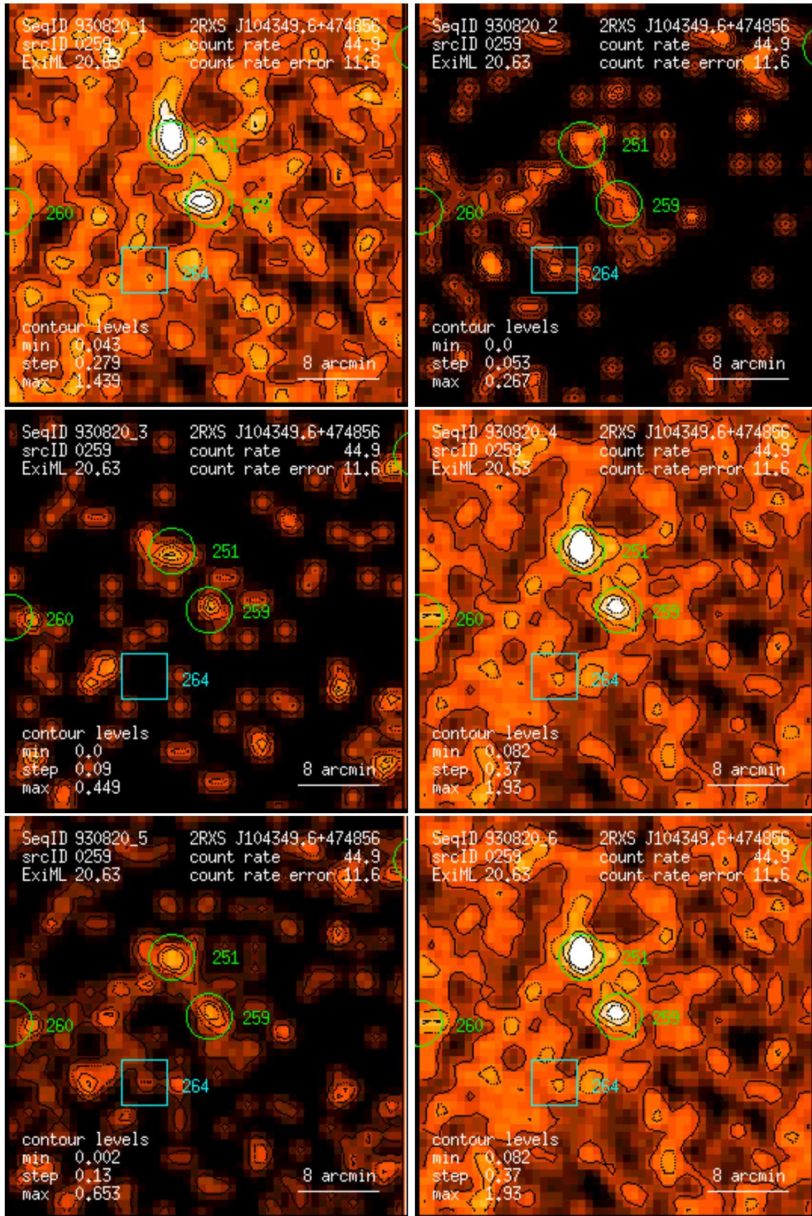
Figure 259: RASS 930820: detection 0259: band rate images, Gaussian filter: (1) PSPC channels 11 – 41, (2) 52 – 90, (3) 91 – 201, (4) 11 – 235, (5) 52 – 201, (6) 11 – 201. Broad band rates in counts/ks. Band rate contour levels in counts/ks/arcmin 2 .
