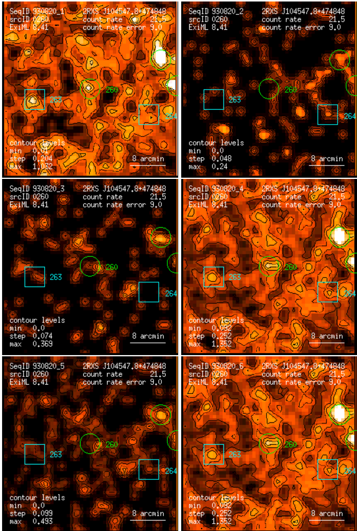
Figure 260: RASS 930820: detection 0260: band rate images, Gaussian filter: (1) PSPC channels 11 – 41, (2) 52 – 90, (3) 91 – 201, (4) 11 – 235, (5) 52 – 201, (6) 11 – 201. Broad band rates in counts/ks. Band rate contour levels in counts/ks/arcmin 2 .
